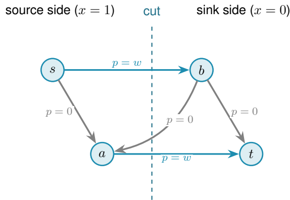
Figure 2.8. One chosen s - t cut. Only the two thick source-to-sink arcs contribute crossing weight p = w , while same-side and backward arcs have p = 0 .
