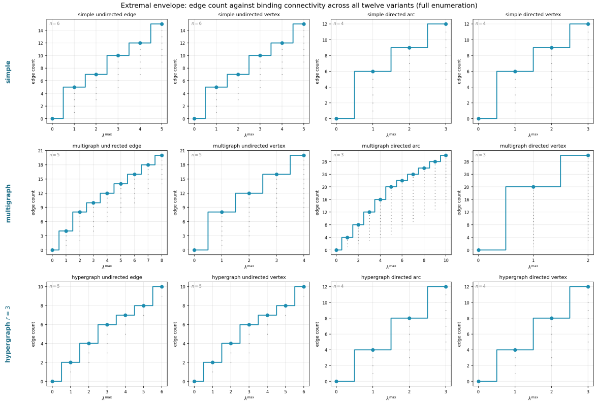
Figure 4.4. The complete landscape of all labeled graphs at small n (see panel annotations for each variant's n ): every point is one graph, plotted at its binding connectivity \lambda^{\max} horizontally and its edge count vertically. The blue staircase marking the densest graph at each connectivity level is the extremal envelope, the frontier the extremal problem asks about, with one dot per level so its exact value is legible. Graphs crowd the low-connectivity, low-edge region. The extremal graphs live at the top of the staircase. The emptiness above the envelope is exactly the region the main theorems forbid.
