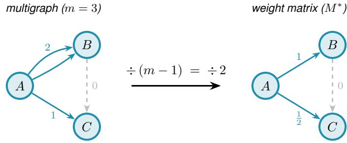
Figure 2.5. The scaling step for m = 3 . Dividing each multiplicity by m - 1 = 2 maps the integer multigraph (left) to a weight matrix with all values in [0, 1] and max-flow at most one between every pair (right). The double arc A \rightarrow B (multiplicity 2) becomes weight 1; the single arc A \rightarrow C (multiplicity 1) becomes weight \frac{1}{2} ; the absent arc B \rightarrow C (multiplicity 0, shown dashed) stays absent. Crucially, m drops out on the right, so a single optimisation over all weight matrices pins L_m^{\text{dir}}(n) = (m - 1) M^*(n) for every m simultaneously.
