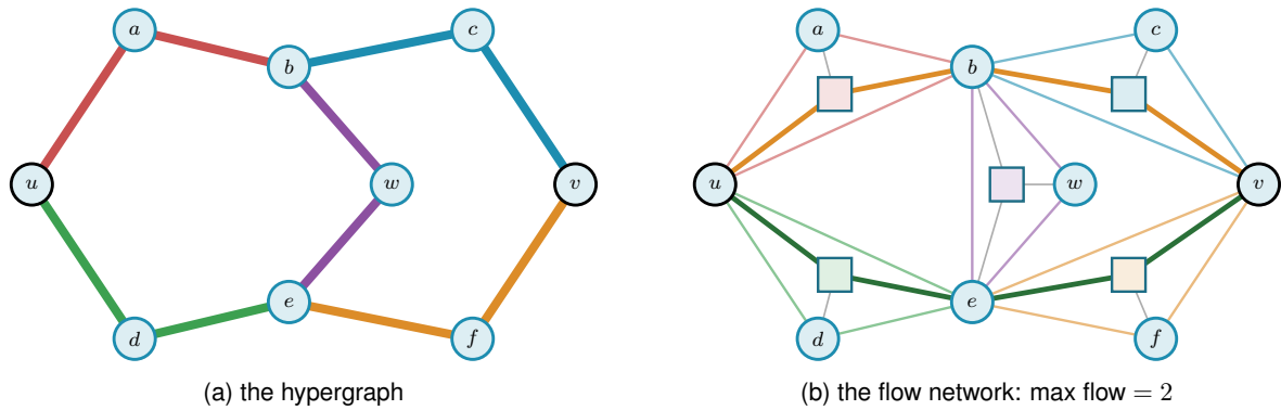
Figure 2.6. From hypergraph to flow network, before and after. (a) A hypergraph on nine vertices, its five hyperedges drawn as metro lines whose triangles do not overlap. The pair u, v has two hyperedge-disjoint Berge routes, u, e_1, b, e_2, v and u, e_3, e, e_4, v . (b) The same vertices, with one helper square sitting inside each hyperedge's triangle (a turnstile on the line). Each Berge route becomes a flow path that enters a line through one member, crosses its helper, and leaves through another: u \rightarrow h_{e_1} \rightarrow b \rightarrow h_{e_2} \rightarrow v (orange) and u \rightarrow h_{e_3} \rightarrow e \rightarrow h_{e_4} \rightarrow v (green). Because every helper carries only one unit, the maximum u - v flow is exactly two, which the checker reports as \lambda(u, v) = 2 . A third route would have to reuse a helper.
