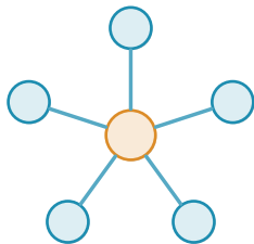
tree
