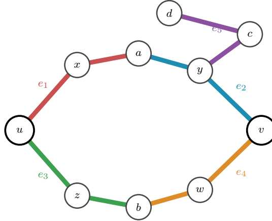
Figure 1.9. A three-uniform hypergraph on ten vertices, its five hyperedges drawn as metro lines. To travel from u to v one rides a line and changes at a shared station. Route A takes the red line e_1 to a and changes there to the blue line e_2 into v ; route B takes the green line e_3 to b and changes to the orange line e_4 . The two journeys share no line, so they are hyperedge-disjoint Berge routes and \lambda(u, v) \geq 2 . A third route would have to reuse a line already taken. Just as a metro line carries one train past a point at a time, a whole hyperedge, not a single edge, is what each route consumes.
