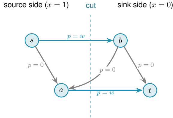
Figure A.4. One chosen s – t cut. Only the two thick source-to-sink arcs contribute crossing weight p = w , while same-side and backward arcs have p = 0 .
