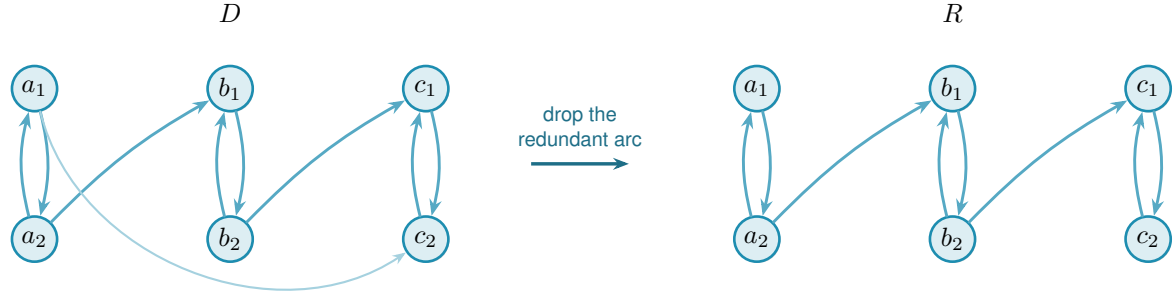
Figure A.3. A small instance of Lemma A.38. In D (left) three bidirected pairs A = \{a_1, a_2\} , B = \{b_1, b_2\} , C = \{c_1, c_2\} are the strongly connected components, joined by a_2 \rightarrow b_1 , b_2 \rightarrow c_1 , and a_1 \rightarrow c_2 . Contracting each pair to a point gives a condensation Q_0 on three points, carrying all three arcs A \rightarrow B , B \rightarrow C and A \rightarrow C . That is exactly the transitively-closed triangle the proof rules out of the thinned Q . The arc A \rightarrow C is redundant, since A already reaches C through B , so the transitive reduction Q keeps only A \rightarrow B and B \rightarrow C . The underlying graph of Q is then a path on three points, triangle-free as claimed. The reachability skeleton R (right) reflects exactly this: every SCC keeps both of its internal arcs (an in- and an out-arborescence on two vertices is just the pair itself), while of the two component-crossing arcs of D only the two witnesses of Q 's two arcs survive. The direct arc a_1 \rightarrow c_2 is dropped, yet a_1 still reaches c_2 in R : first a_1 \rightarrow a_2 , then a_2 \rightarrow b_1 , then b_1 \rightarrow b_2 , then b_2 \rightarrow c_1 , then c_1 \rightarrow c_2 .
