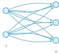
thickened one-way bipartite digraph
