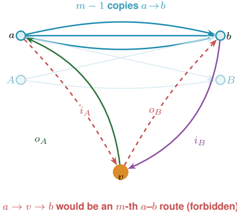
Figure A.4. The attachment lemma (Lemma A.26): a new vertex v is glued onto (m-1) \cdot B_{p,q} , the one-directional complete bipartite multigraph in which every a \in A sends m-1 parallel arcs to every b \in B (the bundle along the top, faint for the pairs other than a, b ). The arcs at v fall into four classes by direction and side: i_A into v from A , o_A out of v to A , i_B into v from B , and o_B out of v to B . The two red legs i_A and o_B are drawn together because they are the worst case: the route a \rightarrow v \rightarrow b laid on top of the m-1 existing a \rightarrow b arcs is an m -th arc-disjoint a - b route, so \lambda(a, b) \geq m , which feasibility forbids. Ruling this out, with two siblings like it, caps d(v) \leq (m-1)\max(p, q) .
