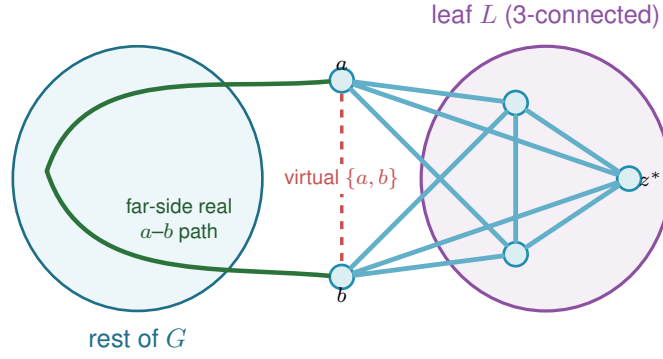
Figure A.7. The triconnected (Tutte/SPQR) decomposition in Step 4 of Lemma A.36 , schematic: G splits into a tree of pieces (blobs) glued along virtual edges, and the analysis works at a leaf L with its single virtual edge \{a, b\} (dashed red). The far side of the tree supplies a real a - b path (green) that internally avoids L . If L is 3-connected, any two of its vertices are joined by three internally disjoint paths inside L , at most one using the virtual edge, and the far-side path replaces it, so \kappa_G \geq 3 for every pair in L . With |V(L)| \geq 4 that forces a hyperedge-node z^* \notin \{a, b\} of degree at most one, which is the contradiction that closes the lemma.
