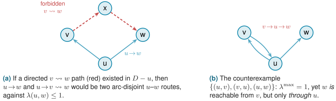
Figure A.3. Why Proposition A.20 must exclude paths through u . (a) For out-neighbours v, w of u in a digraph with \lambda^{\max} \leq 1 , no v \rightsquigarrow w path can avoid u : such a path would combine with the lone arc u \rightarrow w into two arc-disjoint routes. (b) The restriction to D - u is essential. In the three-vertex digraph \{(u, v), (v, u), (u, w)\} we have \lambda^{\max} = 1 , yet v reaches w via v \rightarrow u \rightarrow w , a route that reuses the vertex u , which the proposition allows.
