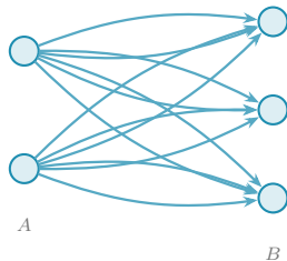
thickened one-way bipartite digraph
