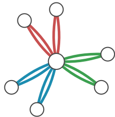
star hypertree, edges repeated m - 1 times
