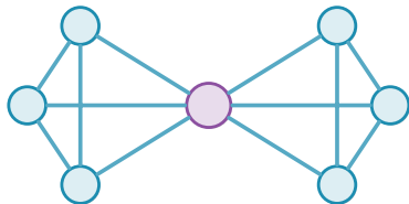
2-connected blocks at a cut vertex
