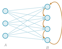
augmented bipartite digraph
