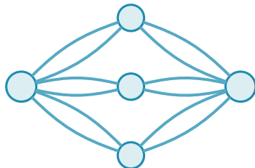
thickened complete bipartite block
