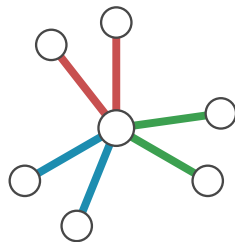
star hypertree ( m = 2 ) EXTREMAL
