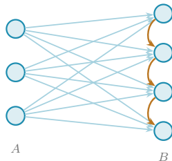
augmented bipartite digraph
