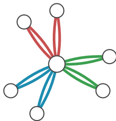
repeated star hypertree EXTREMAL
