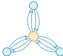
bidirected star, doubled arcs L_3^{\text{dir}}(4) = 12
