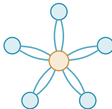
multigraph star L_3(6) = 10
