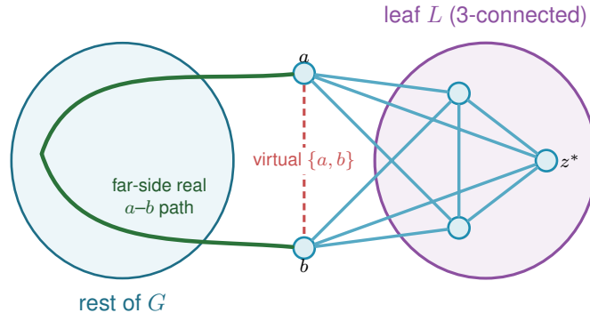
Figure A.6. The triconnected (Tutte/SPQR) decomposition in Step 4 of Lemma A.52 , schematic: G splits into a tree of pieces (blobs) glued along virtual edges, and the analysis works at a leaf L with its single virtual edge \{a, b\} (dashed red). The far side of the tree supplies a real a - b path (green) that internally avoids L . If L is 3-connected, any two of its vertices are joined by three internally disjoint paths inside L , at most one using the virtual edge, and the far-side path replaces it, so \kappa_G \geq 3 for every pair in L . With |V(L)| \geq 4 that forces a hyperedge-node z^* \notin \{a, b\} of degree at most one, which is the contradiction that closes the lemma.
