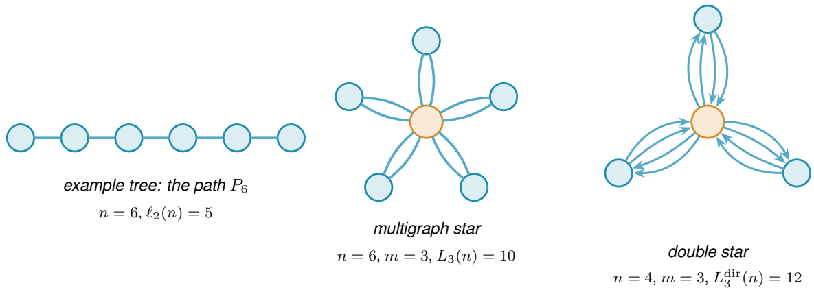
Figure 2.8. Examples from the extremal families discussed alongside Table 2.3 , drawn at the reported sizes. The path illustrates the tree family but is not the saved search witness. Figure 1.7 shows a bidirected star, which ties the one-directional wall at n = 7 .
