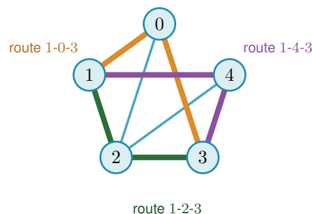
Figure 1.1. A simple graph on five vertices. It is K_5 , the complete graph in which every one of the \binom{5}{2} = 10 pairs is joined by an edge, with the two edges \{0, 4\} and \{1, 3\} removed, so its edge set E(G) holds eight edges. The five dots are the vertex set V(G) and the lines are the edges. The pair 1, 3 carries no edge of its own, yet three routes still join them with no shared edge, 1-0-3 (orange), 1-2-3 (green), and 1-4-3 (purple), each through a different middle vertex, so its local edge-connectivity, defined just below, is \lambda(1, 3) = 3 . Since at most one line joins any given pair and no edge loops back to its own endpoint, this is a simple graph.
