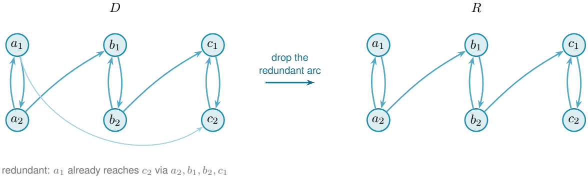
Figure A.3. A small instance of Lemma A.35 . In D (left) three bidirected pairs A = \{a_1, a_2\} , B = \{b_1, b_2\} , C = \{c_1, c_2\} are the strongly connected components, joined by a_2 \rightarrow b_1 , b_2 \rightarrow c_1 , and a_1 \rightarrow c_2 . Contracting each pair to a point gives a condensation Q_0 on three points, carrying all three arcs A \rightarrow B , B \rightarrow C and A \rightarrow C . That is exactly the transitively-closed triangle the proof rules out of the thinned Q . The arc A \rightarrow C is redundant, since A already reaches C through B , so the transitive reduction Q keeps only A \rightarrow B and B \rightarrow C . The underlying graph of Q is then a path on three points, triangle-free as claimed. The reachability skeleton R (right) reflects exactly this: every SCC keeps both of its internal arcs (an in- and an out-arborescence on two vertices is just the pair itself), while of the two component-crossing arcs of D only the two witnesses of Q 's two arcs survive. The direct arc a_1 \rightarrow c_2 is dropped, yet a_1 still reaches c_2 in R : first a_1 \rightarrow a_2 , then a_2 \rightarrow b_1 , then b_1 \rightarrow b_2 , then b_2 \rightarrow c_1 , then c_1 \rightarrow c_2 .
