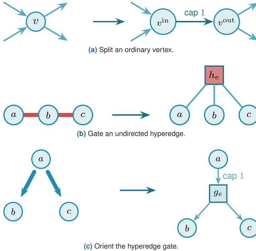
Figure 2.3. The three capacity-one reductions used by the checker. Each forces competing routes through one unit-capacity bottleneck. Direction changes only how the gate is wired.
