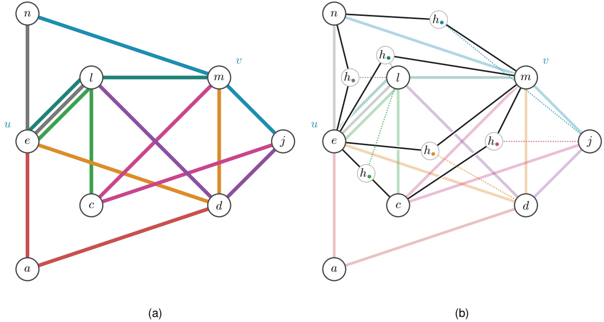
Figure 2.2. An undirected 3-uniform hypergraph and its gate network for u, v . The four black routes use distinct capacity-one gates (they are drawn as one point to reduce visual clutter), so the checker reads \lambda(u, v) = 4 . A fifth would reuse a gate. The helper points connect to the hyperedge's third member by dotted lines.
