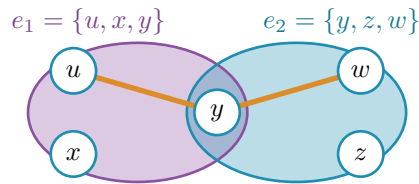
Figure 1.9. A Berge path from u to w in a three-uniform hypergraph, crossing two hyperedges. Each hyperedge (shaded in its own colour) is a set of three vertices, and they meet at the shared vertex y where the two colours blend, and the route (orange) enters e_1 at u and leaves it at y , then enters e_2 at y and leaves it at w . The two steps use distinct hyperedges, so this counts as one Berge path. A second route edge-disjoint from it would have to avoid both e_1 and e_2 entirely. Unlike an ordinary edge, a single hyperedge touches all \binom{3}{2} = 3 pairs of its vertices at once, which is the bookkeeping the checker of Chapter 2 must handle.
