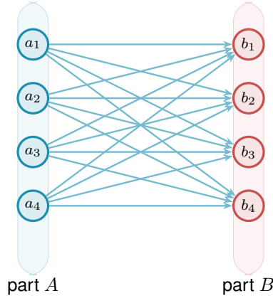
Figure 1.5. The one-directional complete bipartite digraph B_{k,k} of Construction 1.7, drawn here at n = 8 with |A| = |B| = 4 . Every one of the |A| \cdot |B| = \lfloor n^2/4 \rfloor arcs runs left to right, from A to B . There are no arcs inside A , inside B , or back from B to A . Because B has no outgoing arcs and A no incoming ones, the only route from any a_i to any b_j is the single arc a_i \rightarrow b_j , so every pair has local edge-connectivity 1 while the arc count grows quadratically.
