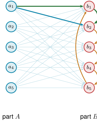
Figure 1.8. The thirty-arc counterexample of Remark 1.11: the augmented bipartite digraph (Construction 1.12) at m = 3 , n = 10 , |A| = |B| = 5 . The 25 faint arcs are the complete one-directional layer from A to B , and the 5 orange arcs form the directed cycle b_1 \rightarrow b_2 \rightarrow b_3 \rightarrow b_4 \rightarrow b_5 \rightarrow b_1 inside B , one extra in-arc per vertex of B . The two heavy arcs and the green path show the pair a_1, b_2 carrying 2 arc-disjoint routes: the direct arc a_1 \rightarrow b_2 (blue) and the detour a_1 \rightarrow b_1 \rightarrow b_2 (green) through the cycle predecessor b_1 . Hence \lambda^{\max} = 2 , feasible at m = 3 , while 30 > \max(3 \cdot 9, 25) = 27 .
