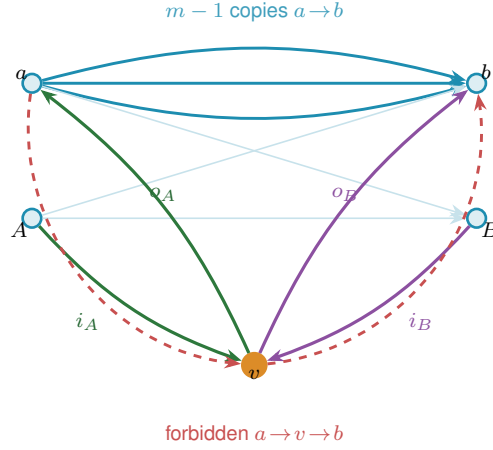
Figure A.4. The attachment lemma (Lemma A.26): the new vertex v glued onto (m - 1) \cdot B_{p,q} . Each a \in A sends m - 1 parallel arcs to each b \in B (the bent bundle). The arcs at v split into four classes by direction and side: i_A (into v from A ), o_A (out of v to A ), i_B , o_B . The red dashed route a \rightarrow v \rightarrow b is forbidden: laid on top of the m - 1 existing a \rightarrow b arcs it makes an m -th arc-disjoint a \rightarrow b route, so \lambda(a, b) \geq m . Ruling out this and two sibling patterns caps d(v) \leq (m - 1) \max(p, q) .
