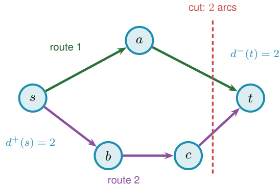
Figure 1.6. The directed measure on one small digraph. The pair (s, t) carries two arc-disjoint directed routes, s \rightarrow a \rightarrow t (green) and s \rightarrow b \rightarrow c \rightarrow t (purple). Deleting the two arcs that enter t separates s from t , so by Menger (Theorem A.1) the local connectivity \lambda(s, t) = 2 equals the size of that minimum arc-cut (red dashed). The degree bound \lambda(s, t) \leq \min(d^+(s), d^-(t)) is tight here, since both out-degree of s and in-degree of t equal 2. Arc-disjoint routes counted against the smallest arc-cut are the whole of what the directed problems measure.
