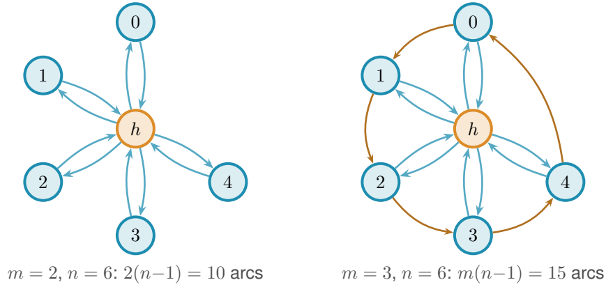
Figure 1.7. The directed hub at n = 6 for two values of m . Left ( m = 2 ): the bidirected star. The hub h is joined to each spoke by one arc in each direction, giving 2(n - 1) = 10 arcs. No circulant layer is added, so all spoke communication routes through h , so \lambda^{\max} = 1 . Right ( m = 3 ): a single circulant layer is added among the five spokes. The blue arcs are the same hub-spoke pairs as on the left. The orange arcs are that one circulant layer, the cycle 0 \rightarrow 1 \rightarrow 2 \rightarrow 3 \rightarrow 4 \rightarrow 0 , so each spoke has d^+ = d^- = m - 1 = 2 . The total is m(n - 1) = 15 arcs and \lambda^{\max} = 2 . For m \geq 3 the spokes are no longer isolated from one another, and tracing all the routes becomes the argument that fills the rest of the chapter.
