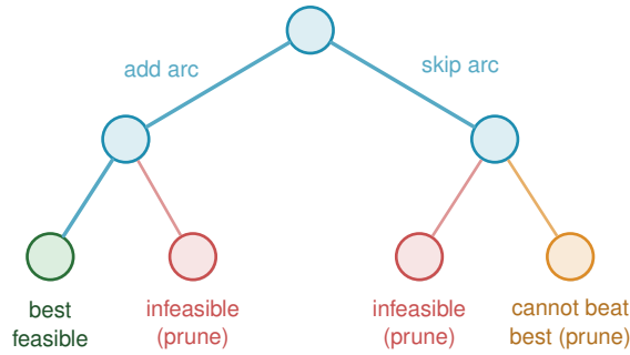
Figure 2.6. Branch and bound over digraphs. Each level fixes one adjacency. Infeasible partial graphs (red) and branches unable to beat the incumbent (orange) are discarded, allowing the exact search to reach n \leq 7 .
