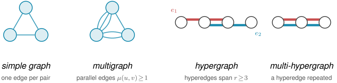
Figure 1.3. The first axis of variation, the model , shown for the four object classes this thesis uses. In a simple graph each pair of vertices is joined by at most one edge. A multigraph permits parallel edges, here a triple and a double, so the multiplicity \mu(u, v) counts how many copies join a pair. A hypergraph replaces pairwise edges by hyperedges, each spanning r \geq 3 vertices and drawn the way a metro map draws a line, threading all of its stations. The red line e_1 and the blue line e_2 share the corridor between two stations, and there the two run side by side, one colour each, exactly as a metro map separates lines that share a stretch of track. A multi-hypergraph lets a hyperedge be repeated, drawn as two parallel lines through the same stations, the hypergraph counterpart of parallel edges. When all hyperedges have the same size r the hypergraph is r -uniform. The same connectivity question, how many independent routes a pair can be forced to share, is asked of all four.
