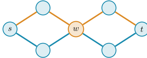
Figure 1.5. The third axis, the separation . The two s – t routes drawn here, one orange and one blue, share no edge, so they count as two edge-disjoint paths and \lambda(s, t) = 2 . Both pass through the single vertex w , however, so they are not internally vertex-disjoint, and since every s – t route must cross w we have \kappa(s, t) = 1 . This is Whitney’s inequality \kappa \leq \lambda made concrete: the gap between the two separations is exactly what the vertex-disjoint problem measures, and the rest of the chapter shows it stays shut until m = 5 .
