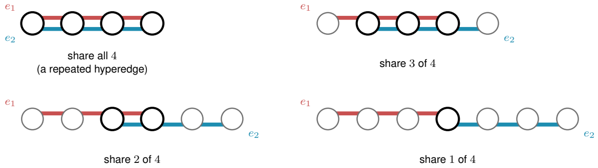
Figure 1.11. Reading hyperedge overlap as a metro map, for r = 4 . Each panel shows two four-vertex hyperedges, the red line e_1 and the blue line e_2 , drawn so that wherever they share consecutive stations the two lines run parallel, side by side, one colour each, exactly as a metro map separates two lines along a shared stretch of track. From top-left to bottom-right the hyperedges share 4, 3, 2, and 1 of their four vertices. Sharing all four (top-left) is a repeated hyperedge, the parallel-edge phenomenon one model up, so it lives only in a multi-hypergraph. Sharing just one (bottom-right) is a single interchange station where the lines meet but never run together. Interchange stations, where both lines stop, are ringed in black. Two Berge routes are hyperedge-disjoint exactly when the lines they ride share no track at all.
