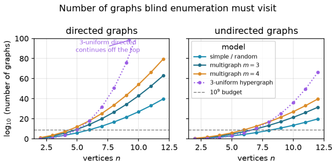
Figure 2.7. Candidate counts for blind enumeration on a logarithmic scale. Every model crosses the generous 10^9 budget in single-digit order, and directed objects grow fastest because they have more independent cells to fill.
