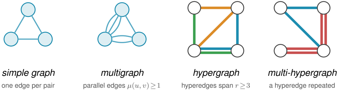
Figure 1.3. The model axis: a simple graph, a multigraph with parallel edges, a 3-uniform hypergraph drawn as metro lines, and a multi-hypergraph with a repeated hyperedge.
