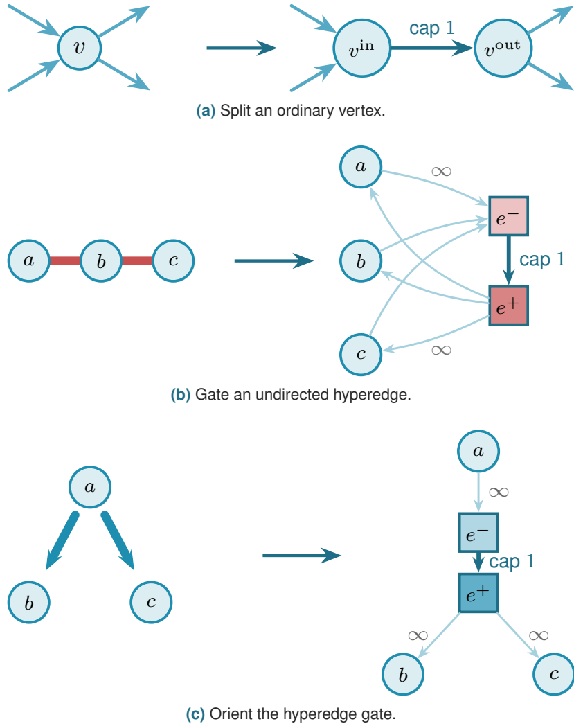
Figure 2.3. The three capacity-one reductions used by the checker. Each forces competing routes through one unit-capacity bottleneck, drawn in dark blue: the internal arc e^- \rightarrow e^+ of the gate, or v^{\text{in}} \rightarrow v^{\text{out}} for a split vertex. The membership arcs joining the gate to the hyperedge's vertices are uncapped, marked \infty . Direction changes only which of them are drawn. Undirected, every member links to the gate both ways. Directed, tails enter e^- and heads leave e^+ .
