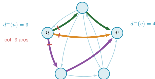
Figure 1.5. Three arc-disjoint u \rightarrow v routes (coloured) and the matching three-arc directed cut (red) in a simple digraph. Thus \lambda(u, v) = 3 , meeting the degree bound \min(d^+(u), d^-(v)) = 3 .
