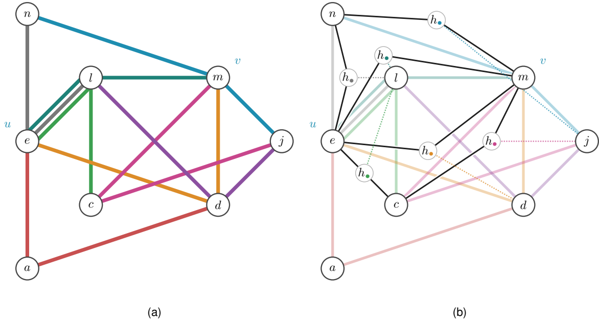
Figure 2.2. An undirected 3-uniform hypergraph and its gate network for u, v . The four black routes use distinct capacity-one gates, so the checker reads \lambda(u, v) = 4 . A fifth would reuse a gate.
