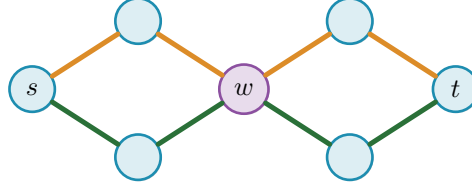
Figure 1.6. The separation axis: two edge-disjoint s – t routes both pass through w , so \lambda(s, t) = 2 but \kappa(s, t) = 1 .
