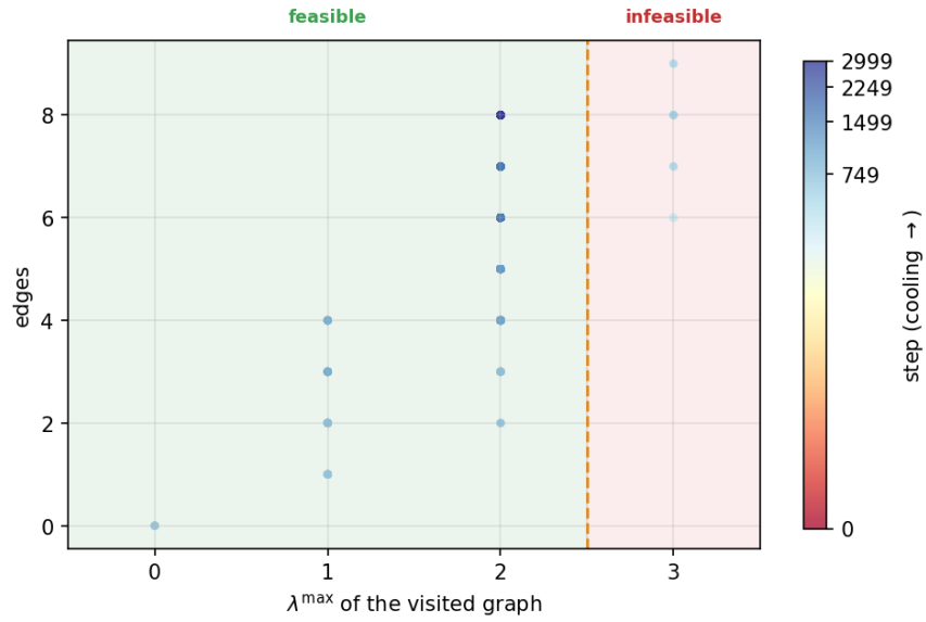
Figure B.4. Search trace for the multigraph undirected edge problem at n = 5, m = 3 . File trace_multi_undirected_n5_m3.png .
