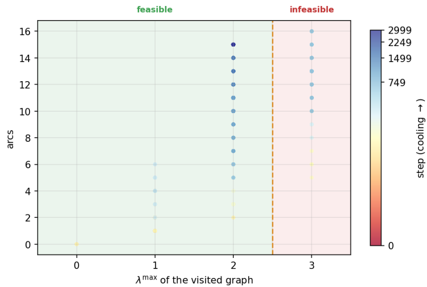
Figure B.5. Search trace for the multigraph directed arc problem at n = 5, m = 3 . File trace_multi_directed_n5_m3.png .
