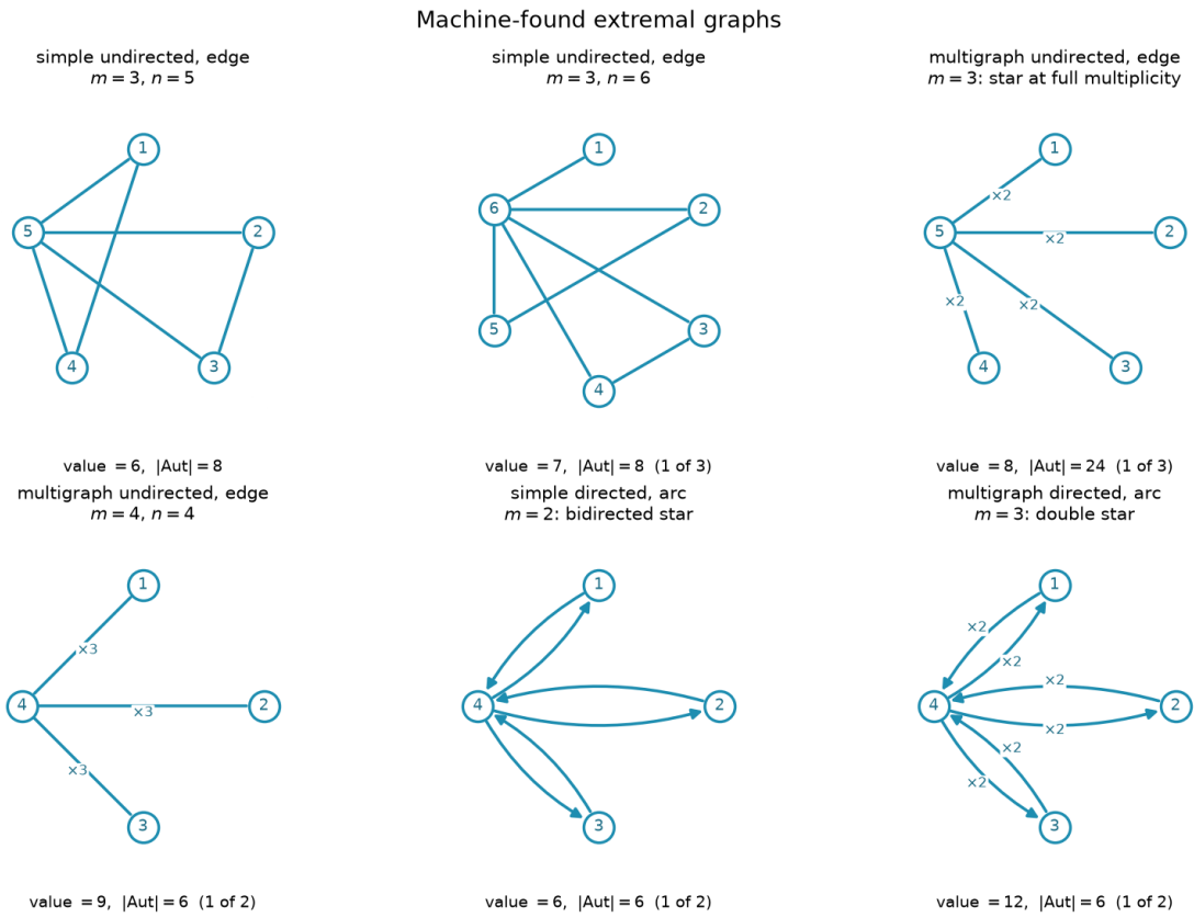
Figure B.1. Machine-found extremal graphs across the matrix variants. Each panel is one densest feasible graph at the stated n and m , drawn from the enumeration output, with its extremal value and automorphism count |\text{Aut}| below it. Edge or arc multiplicities appear as \times k labels, and a note “1 of k ” marks a variant with several non-isomorphic extremisers, of which one is drawn. File extremal_graphs_gallery.png .
