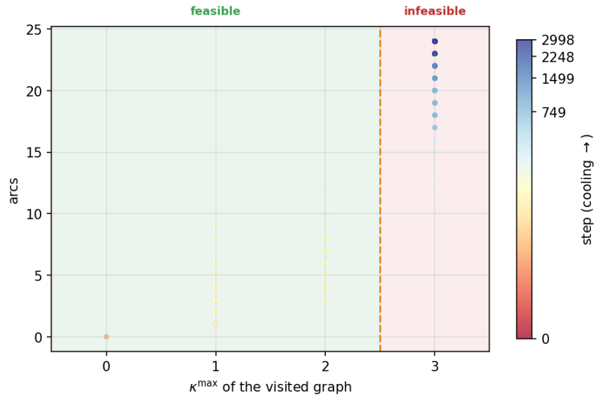
Figure B.6. Search trace for the multigraph directed vertex -disjoint problem at n = 4 , m = 3 , where the binding quantity is \kappa^{\max} . File trace_multi_directed_n4_m3_vertex.png .
