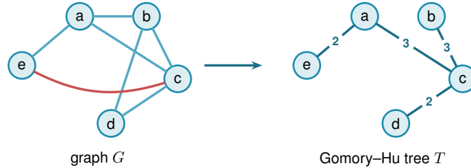
Figure A.1. A graph G and a Gomory–Hu tree T on the same vertices. Each graph edge crosses \text{dist}_T(e) tree cuts, and at most n - 1 edges of a simple graph have tree distance one.
