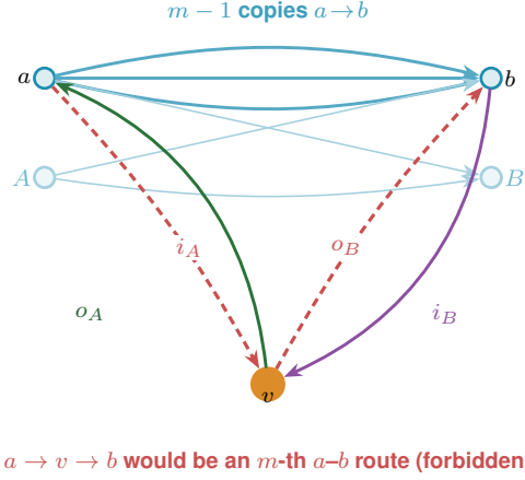
Figure A.4. The attachment lemma (Lemma A.27): a new vertex v is glued onto (m-1) \cdot B_{p,q} , the one-directional complete bipartite multigraph in which every a \in A sends m-1 parallel arcs to every b \in B (the bundle along the top, faint for the pairs other than a, b ). The arcs at v fall into four classes by direction and side: i_A into v from A , o_A out of v to A , i_B into v from B , and o_B out of v to B . The two red legs i_A and o_B are drawn together because they are the worst case: the route a \rightarrow v \rightarrow b laid on top of the m-1 existing a \rightarrow b arcs is an m -th arc-disjoint a - b route, so \lambda(a, b) \geq m , which feasibility forbids. Ruling this out, with two siblings like it, caps d(v) \leq (m-1) \max(p, q) .
