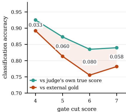
(b) two accuracies, two estimands
