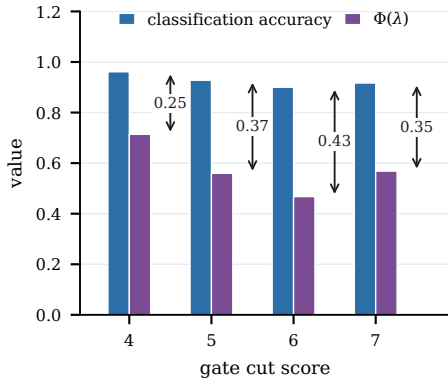
(a) a coefficient is not a probability
