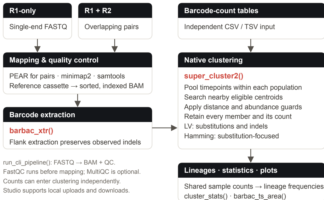
Figure 1. The Barbac workflow. R1-only reads map directly; overlapping paired reads merge with PEAR. Extracted barcodes or independent count tables enter the same native clustering engine. Shared memberships support sample counts, statistics and lineage-frequency plots.
