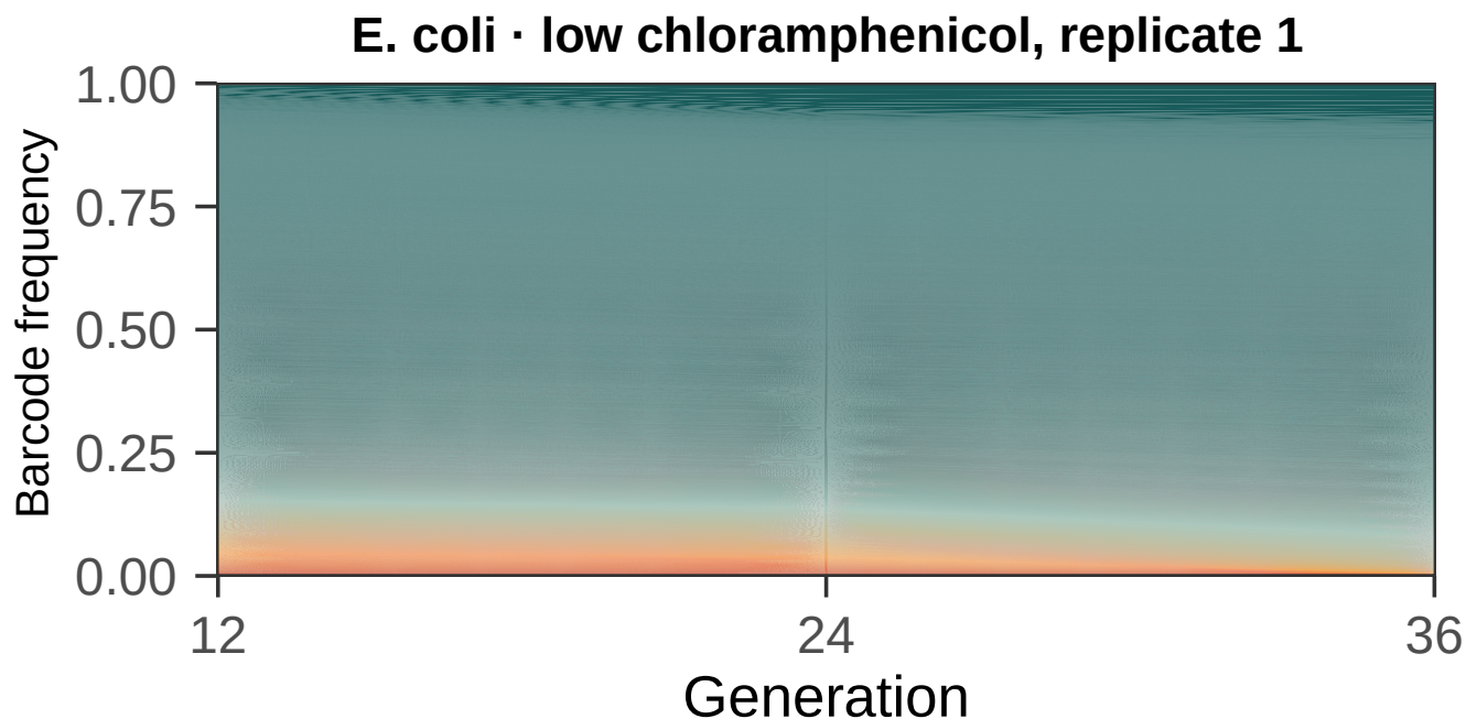
Figure 2. Complete lineage-frequency plot for three E. coli samples (generations 12, 24 and 36), with all 144,537 inferred lineages retained and frequencies normalized to all extracted barcode reads in each sample. Colours distinguish bands rather than biological categories. The saved benchmark data are unchanged; the manuscript shortens the axis label for legibility.
