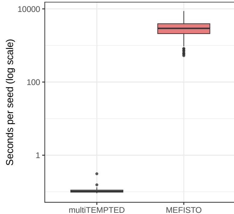
Compute time
