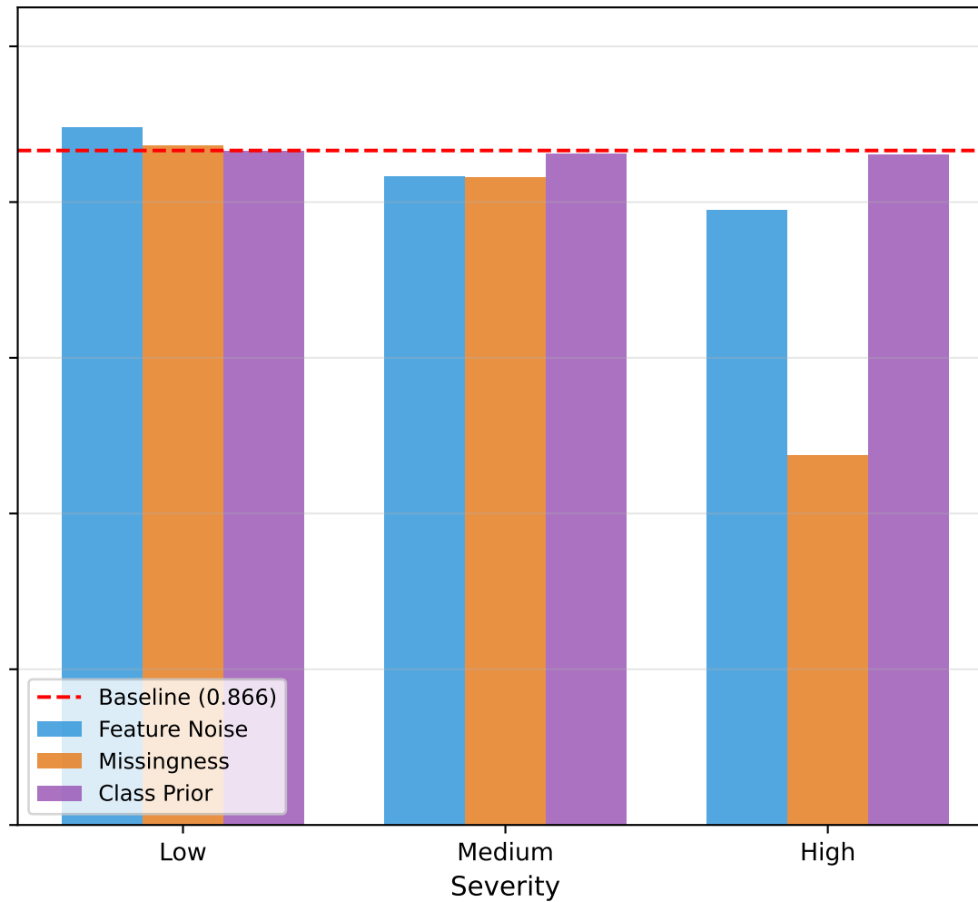
Random Forest
