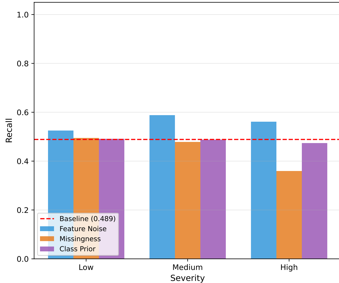
Logistic Regression
