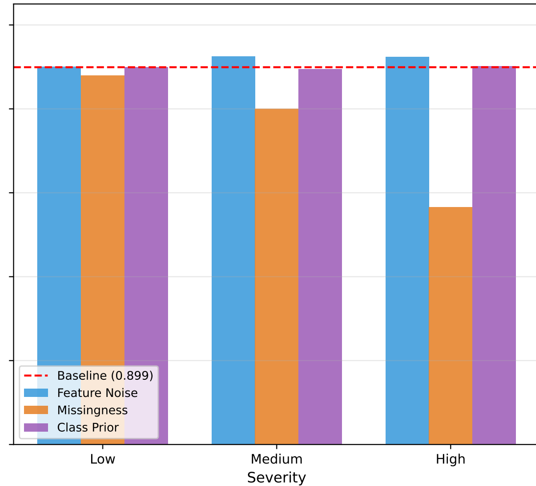
XGBoost
