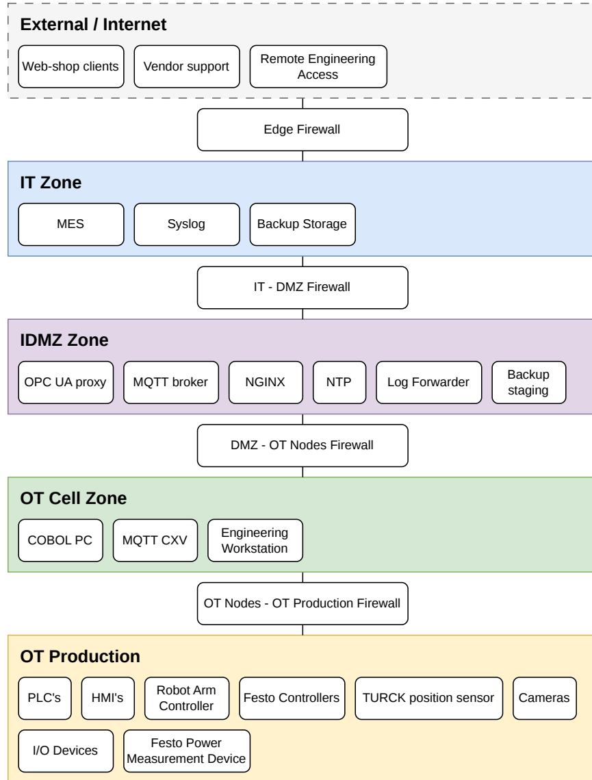
Figure 6.1: Zone & Conduit Diagram
