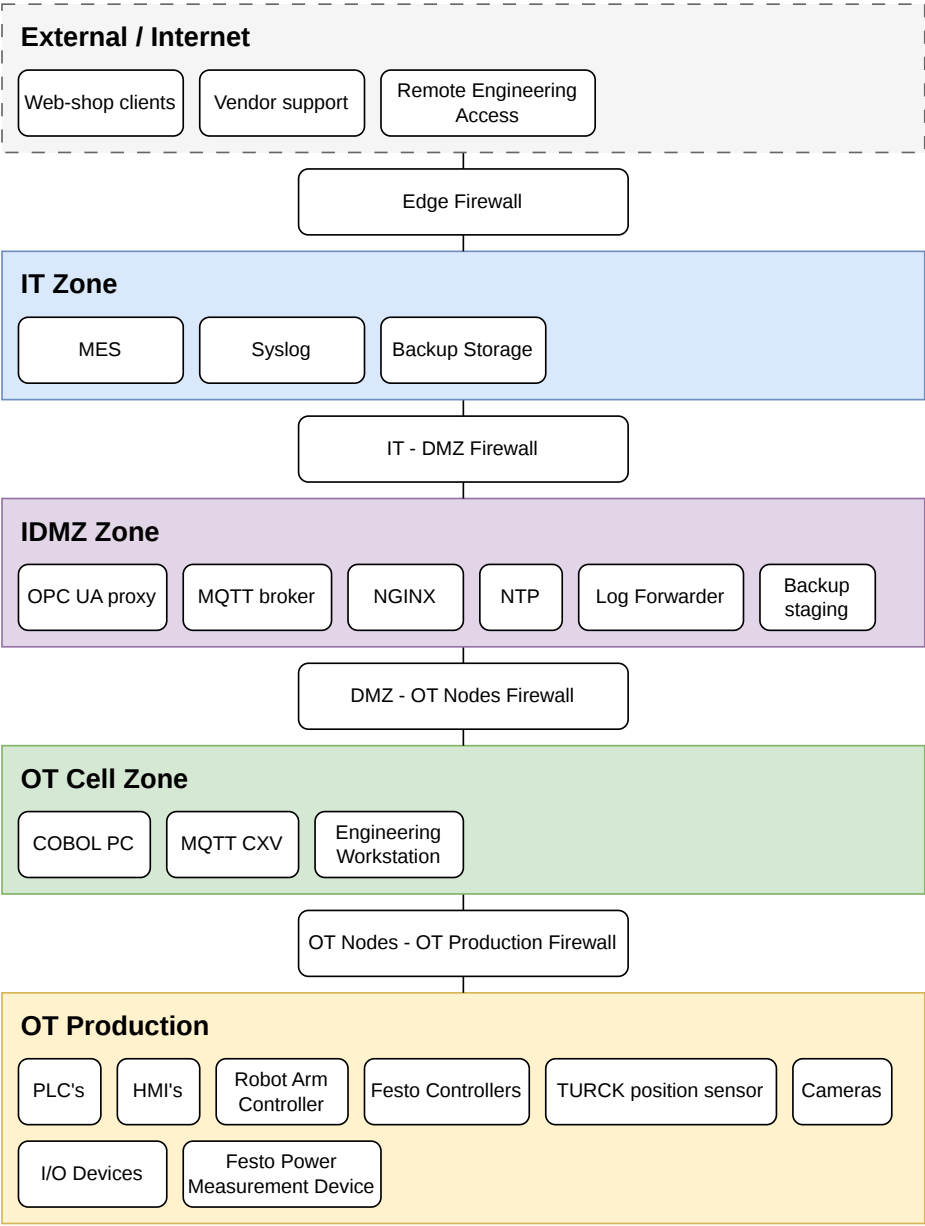
Figure C.1: Zone & Conduit Diagram
