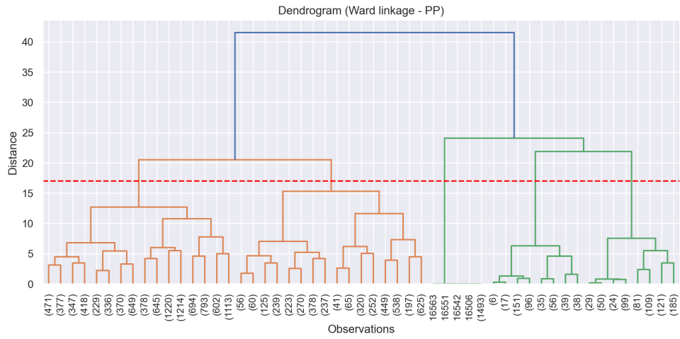
Figure 16: Dendrogram (Ward linkage) for 2nd perspective
