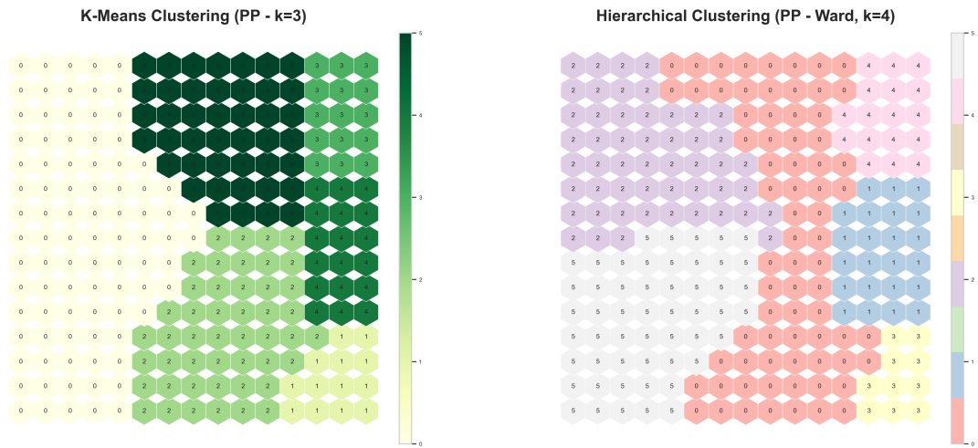
Figure 23: Comparative analysis of SOM with K-Means and HC - 2nd perspective
