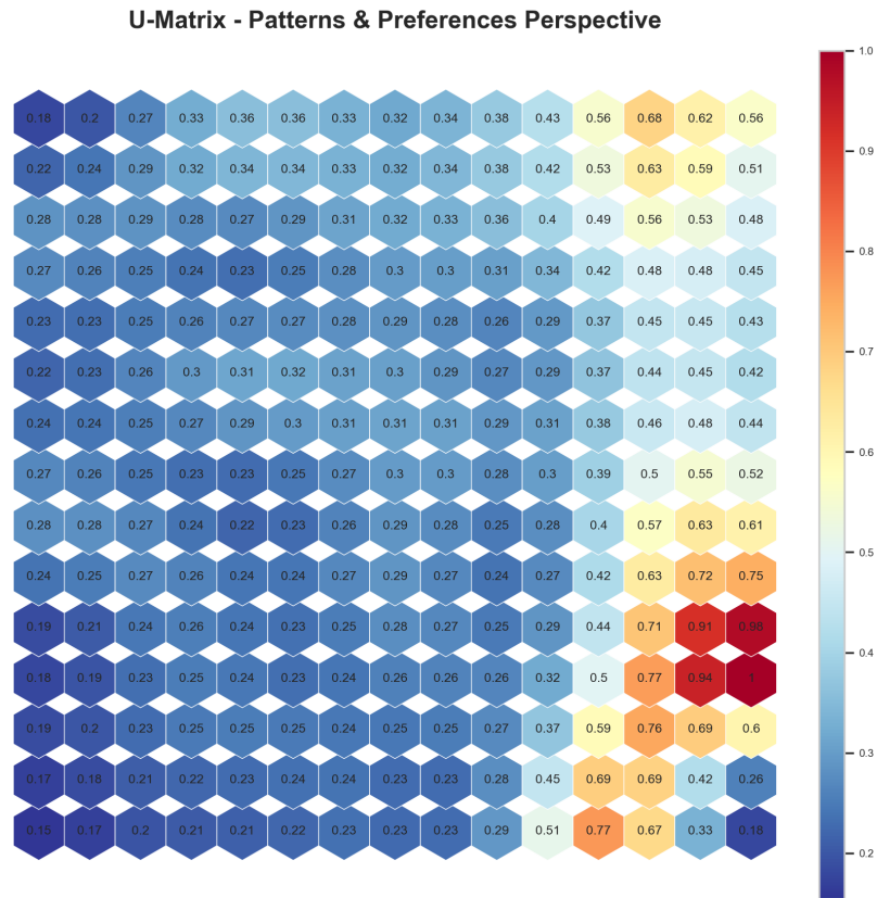
Figure 21: U-Matrix (SOM) for 2nd perspective
