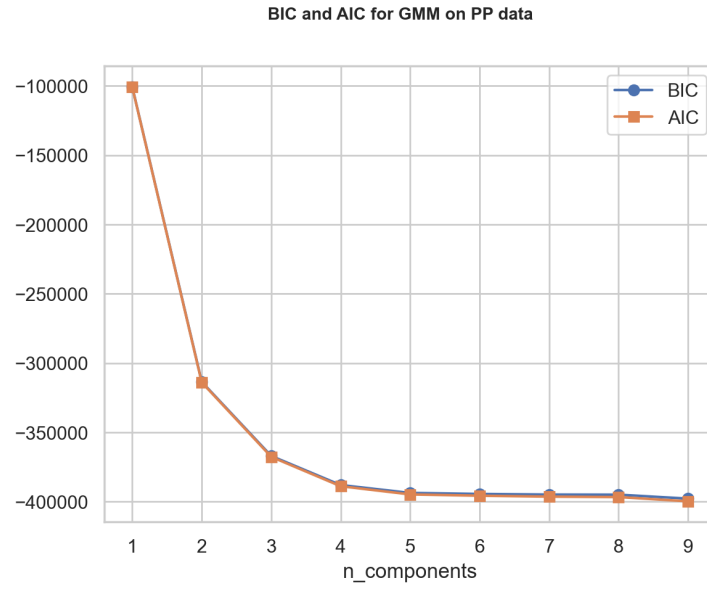
Figure 19: Comparative analysis using BIC and AIC criteria - 2nd perspective
