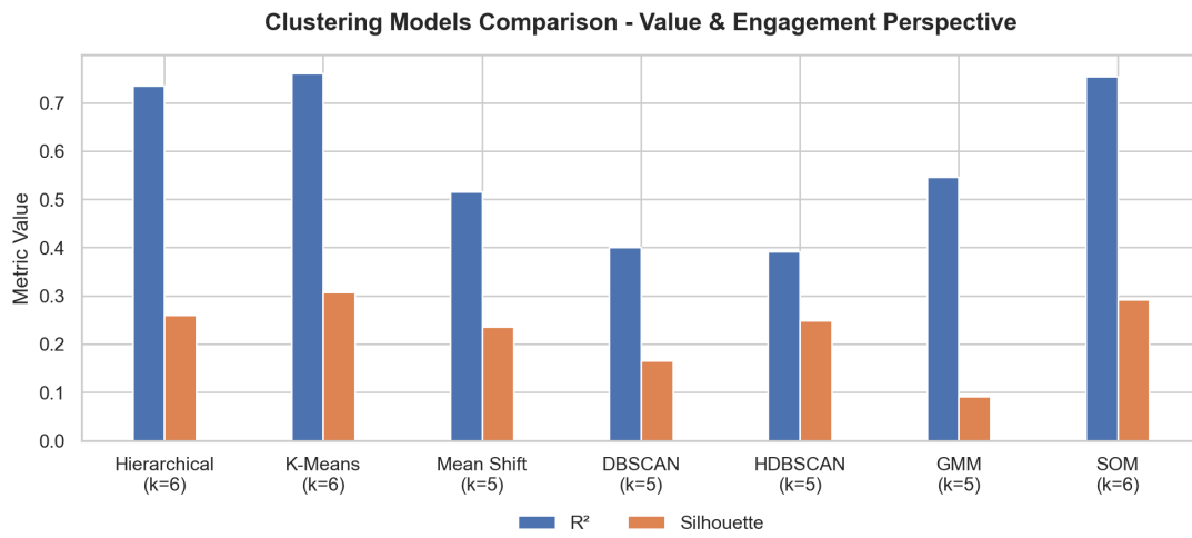
Figure 14: Comparing models for VE perspective
