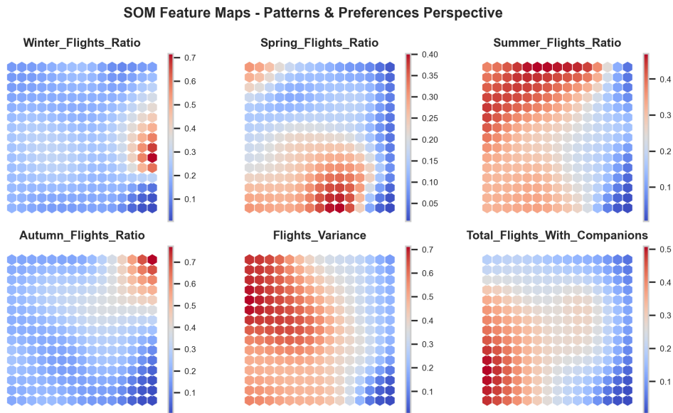
Figure 20: Component Planes (SOM) - 2nd perspective
