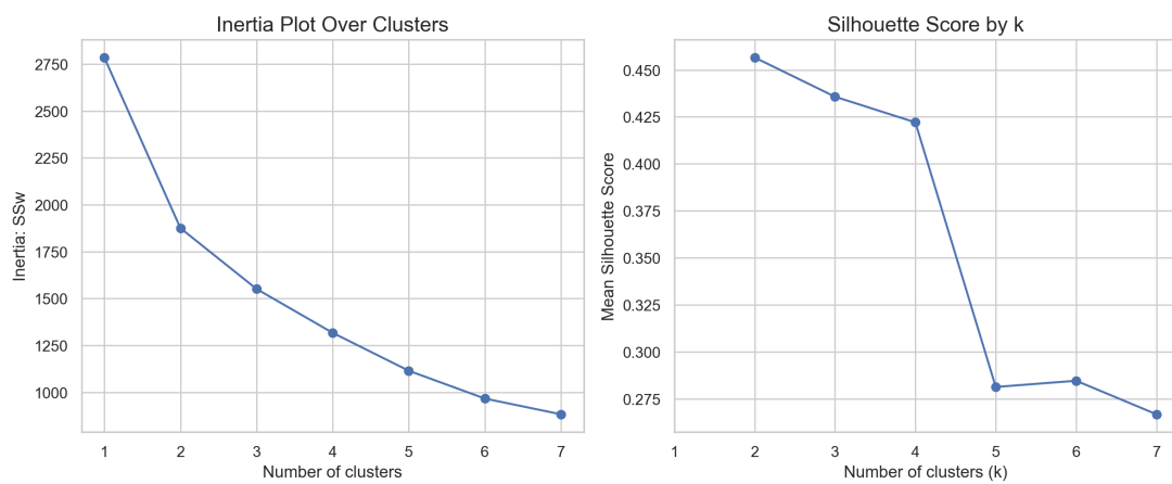
Figure 18: Inertia plot and Silhouette Score (K-Means) for 2nd perspective
