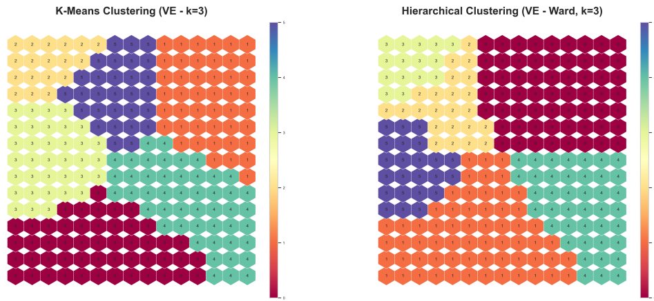
Figure 13: Comparative analysis of SOM with K-Means and HC - VE perspective
