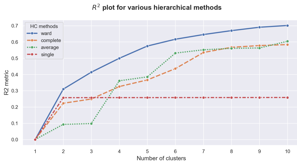
Figure 15: Comparative analysis of R^2 per Hierarchical Method - PP Perspective
