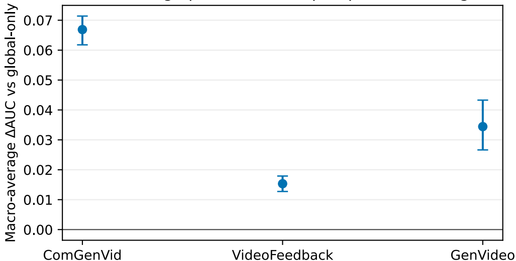
Macro-average paired bootstrap: Alpha-STALLED gains
