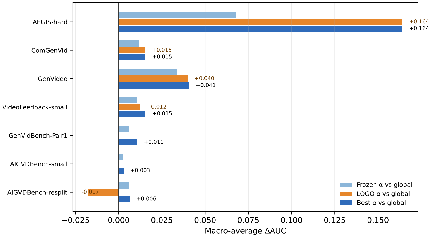
Global-local fusion gains depend on \alpha and dataset
