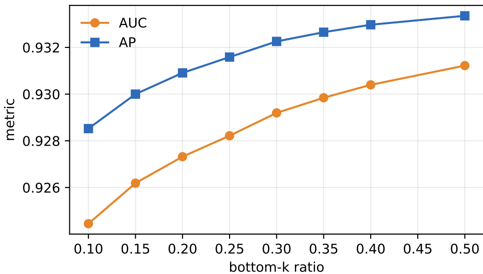
ComGenVid bottom-k ratio
