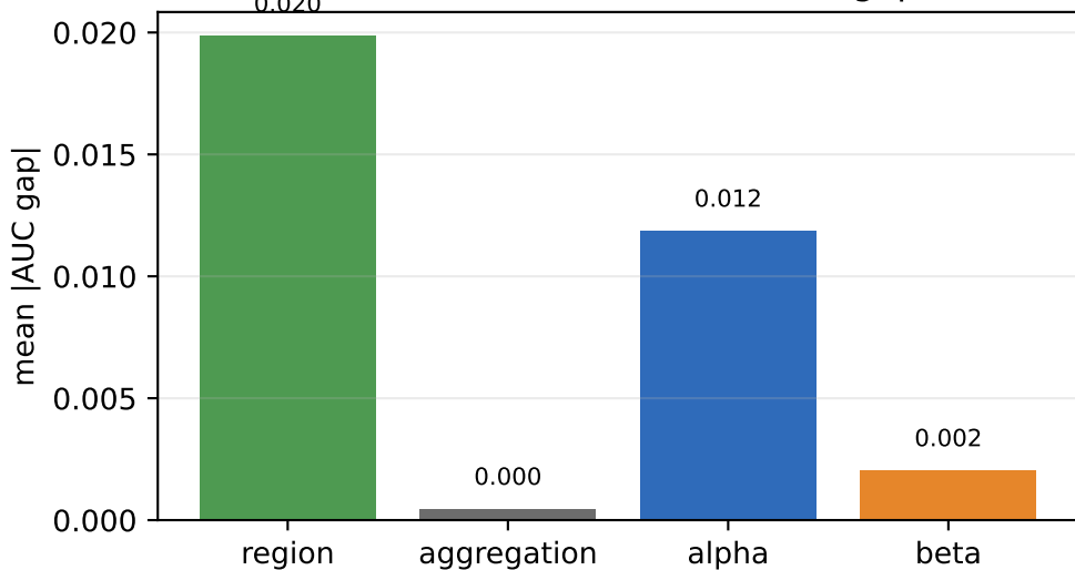
Leave-one-dataset-out oracle gap
