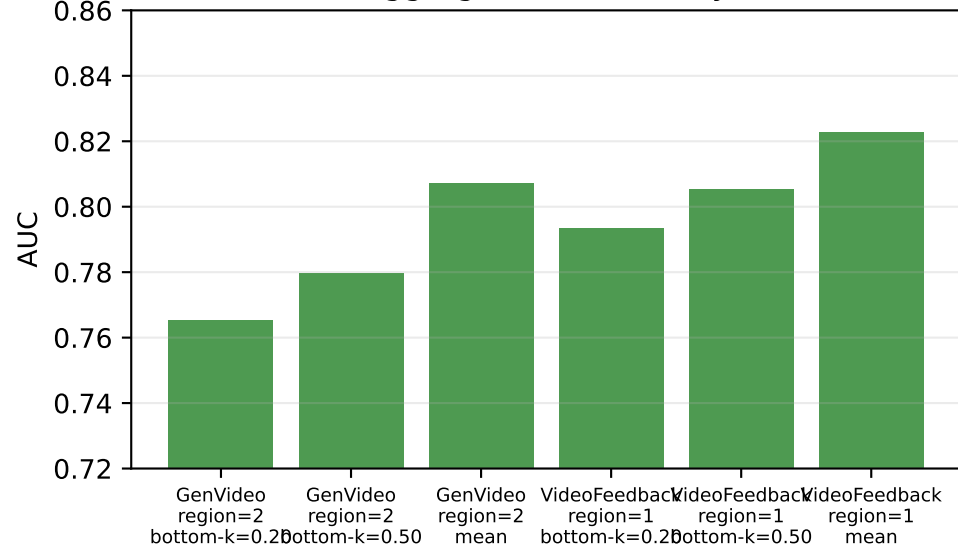
Leave-one-dataset-out oracle gap
