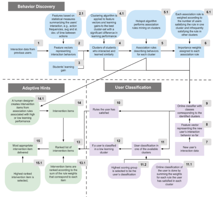
Fig. 9. User Modeling Framework broken down into three phases: Behavior Discovery, User Classification, and Adaptive Hints; rectangular nodes represent inputs and states, oval nodes represent processes.
