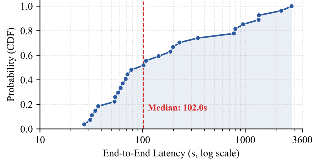
Figure 7: Cumulative Distribution Function (CDF) of end-to-end response latency across 27 CVEs. The x-axis is in log scale to accommodate the long-tail distribution. Over 50% of cases are mitigated within 102 seconds.
