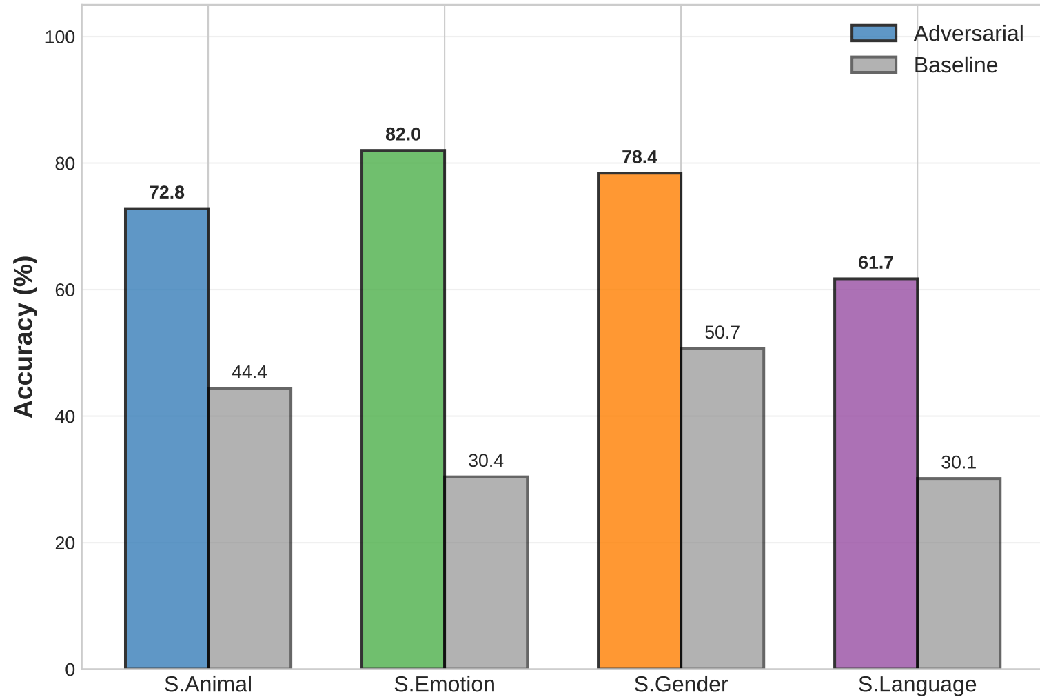
Adversarial Audio Accuracy: Concat + Correct (SALMONN)
