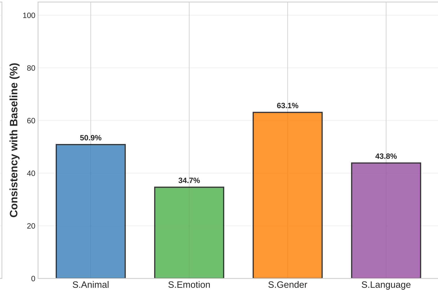
Consistency with Baseline: Concat + Correct (SALMONN)
