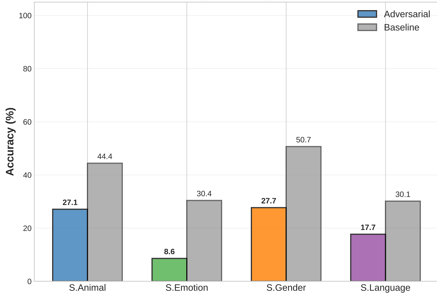
Adversarial Audio Accuracy: Concat + Wrong (SALMONN)
