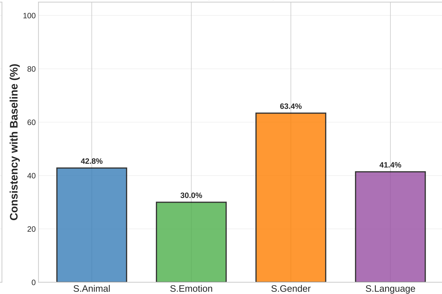
Consistency with Baseline: Concat + Wrong (SALMONN)
