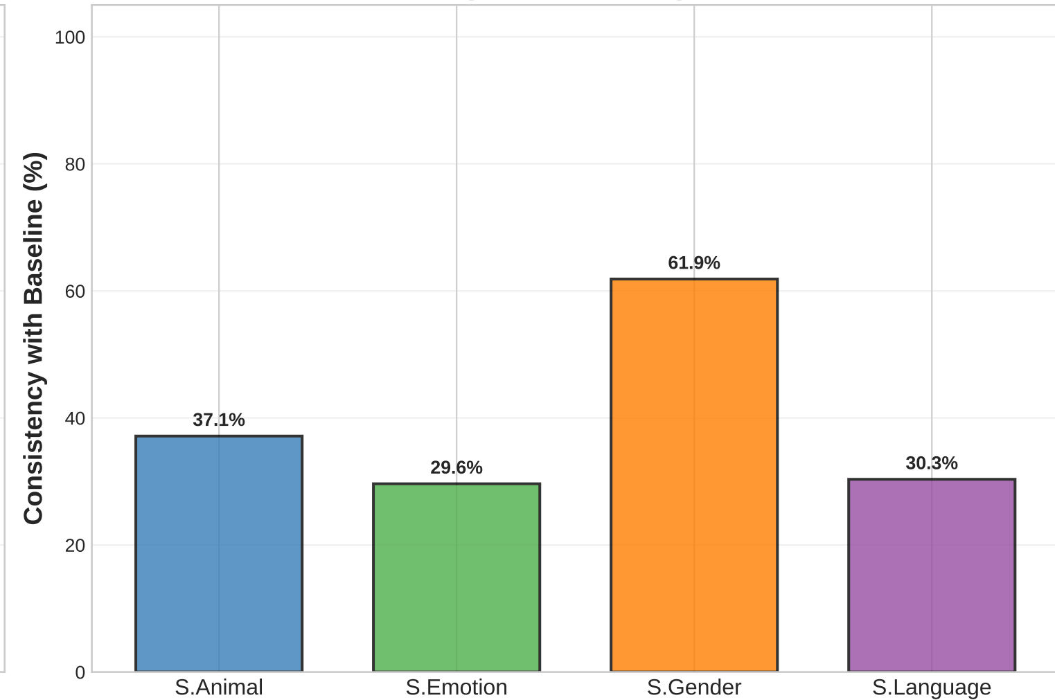
Consistency with Baseline: Concat + Wrong (SALMONN_7B)
