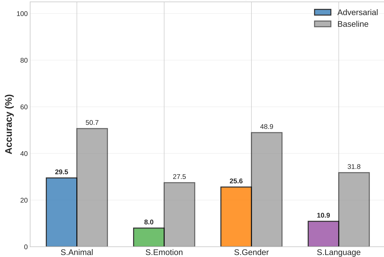
Adversarial Audio Accuracy: Concat + Wrong (SALMONN_7B)
