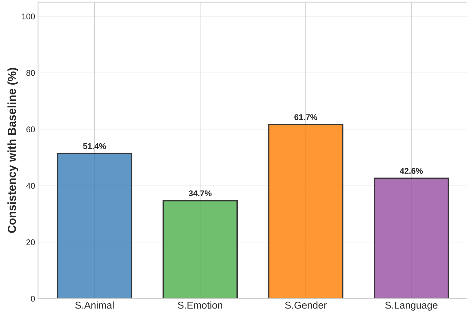
Consistency with Baseline: Overlay + Correct (SALMONN_7B)
