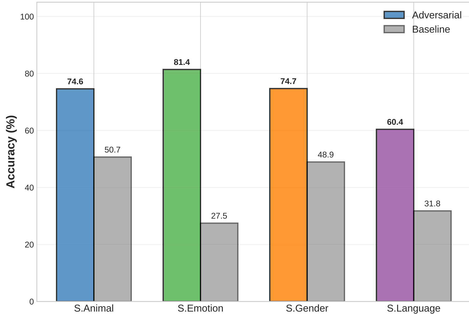
Adversarial Audio Accuracy: Overlay + Correct (SALMONN_7B)
