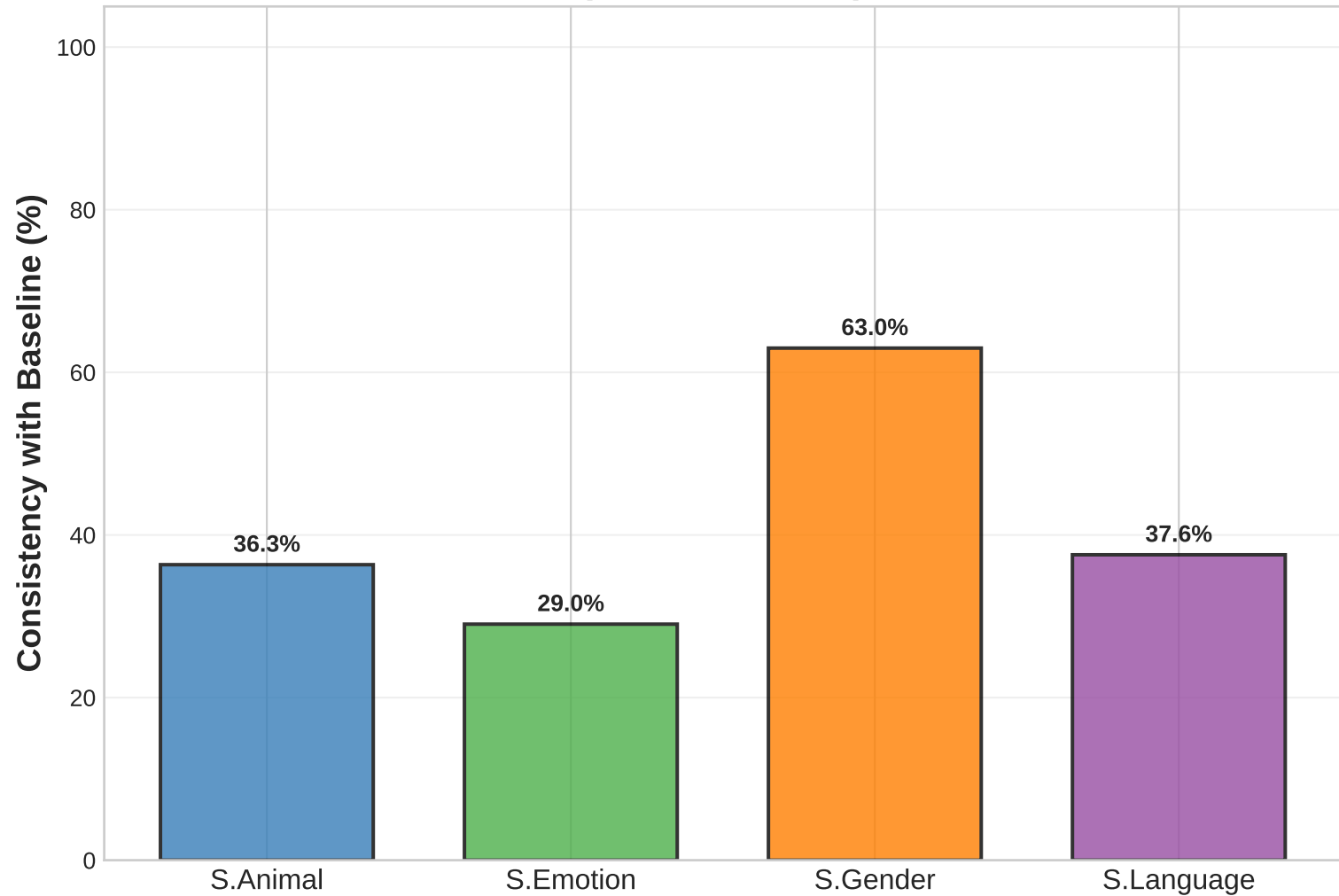
Consistency with Baseline: Overlay + Wrong (SALMONN_7B)
