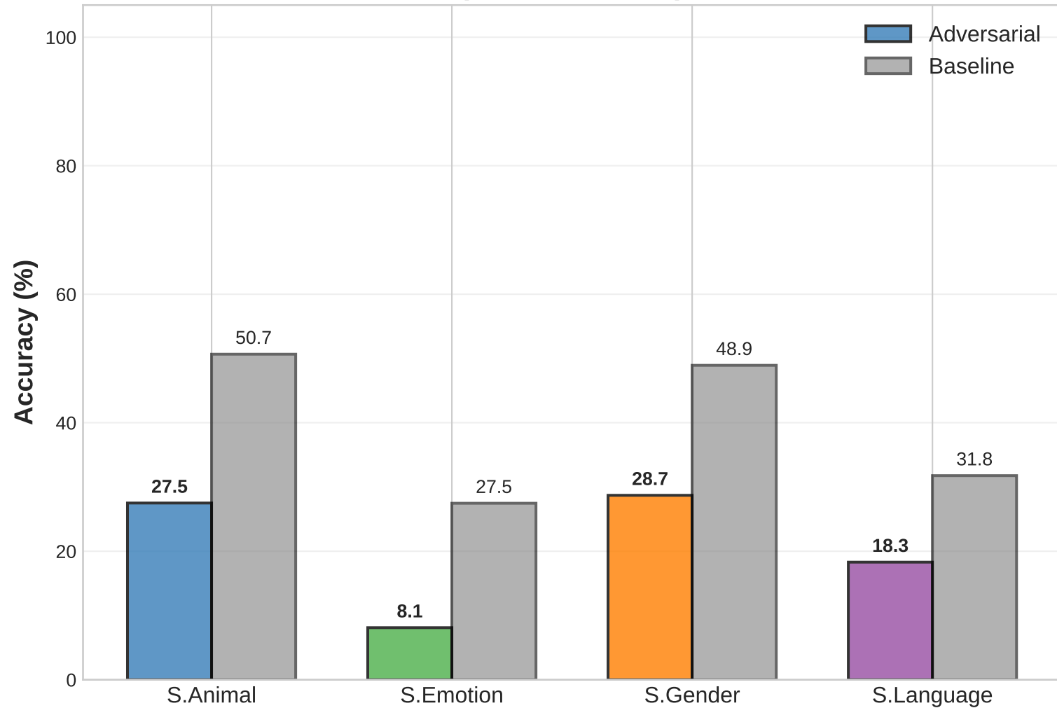
Adversarial Audio Accuracy: Overlay + Wrong (SALMONN_7B)
