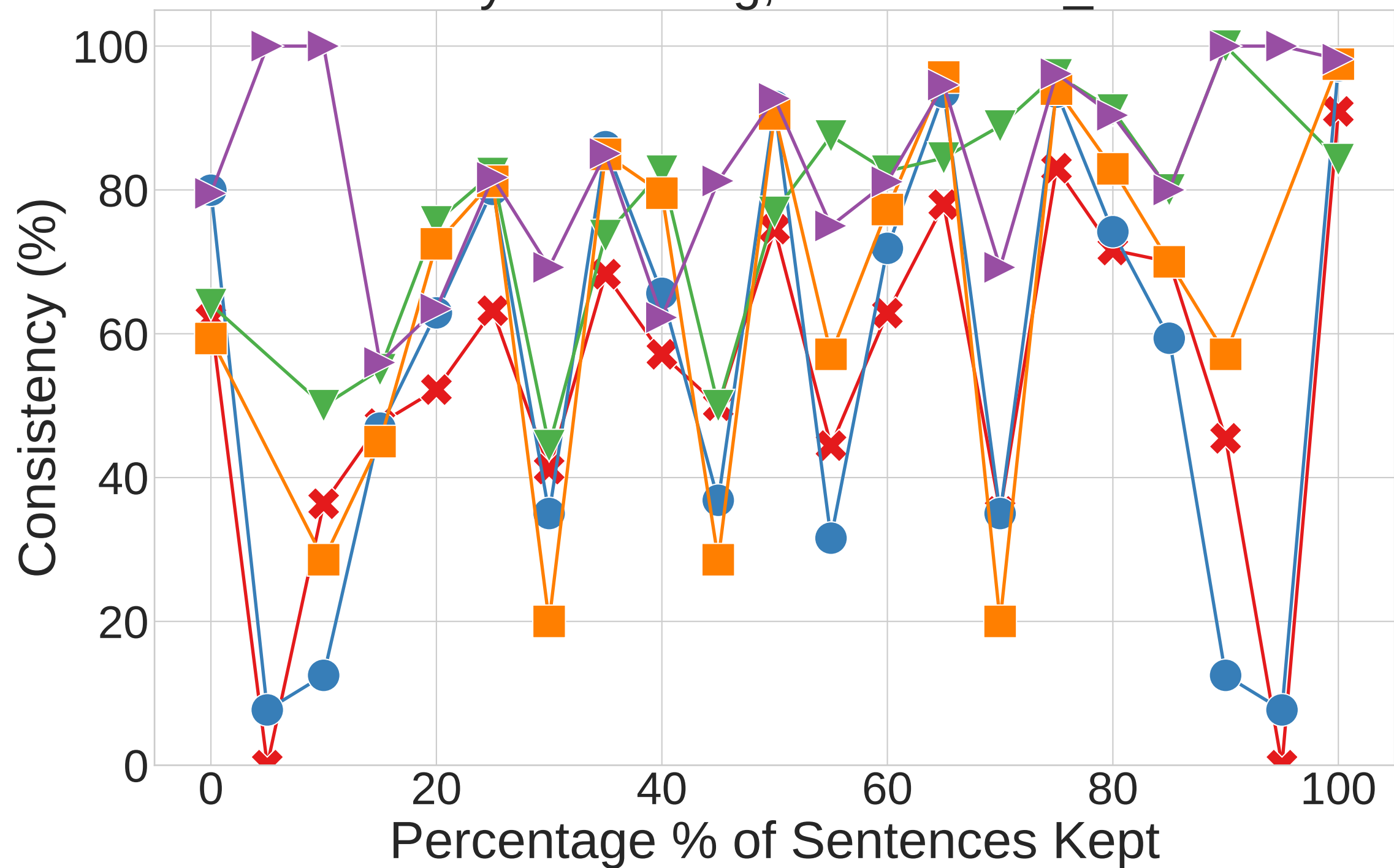
Early Answering, FLAMINGO_HF
