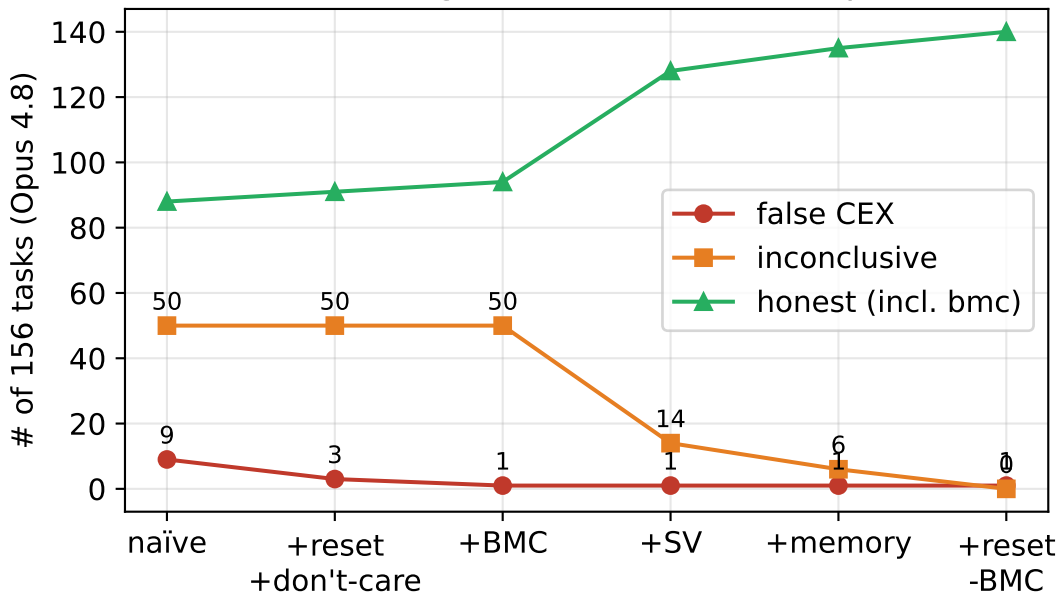
Oracle hardening: artifacts fall, honest pass rises
