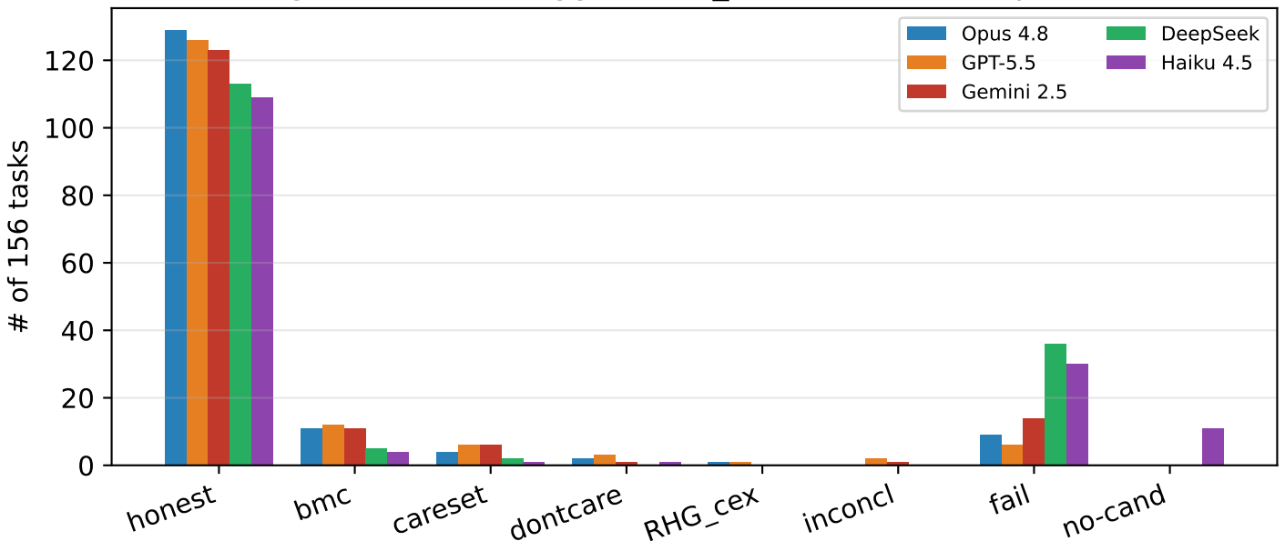
Weakness \neq hacking (5 models): flagged RHG_cex 9→2 (careset-proven; circuit8 residual)
