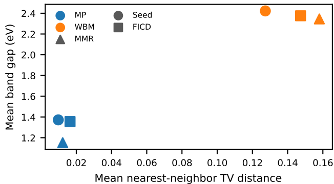
(c) Leave-one-family-out
