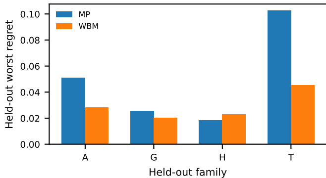
(c) Leave-one-family-out
