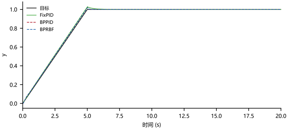
18. Plant3 斜坡跟踪 (0→1)
