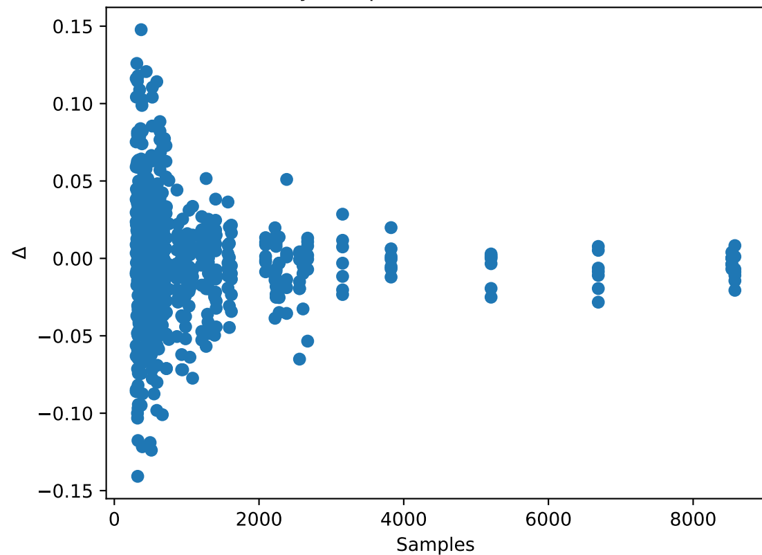
industry Samples vs \Delta - RandomForest
