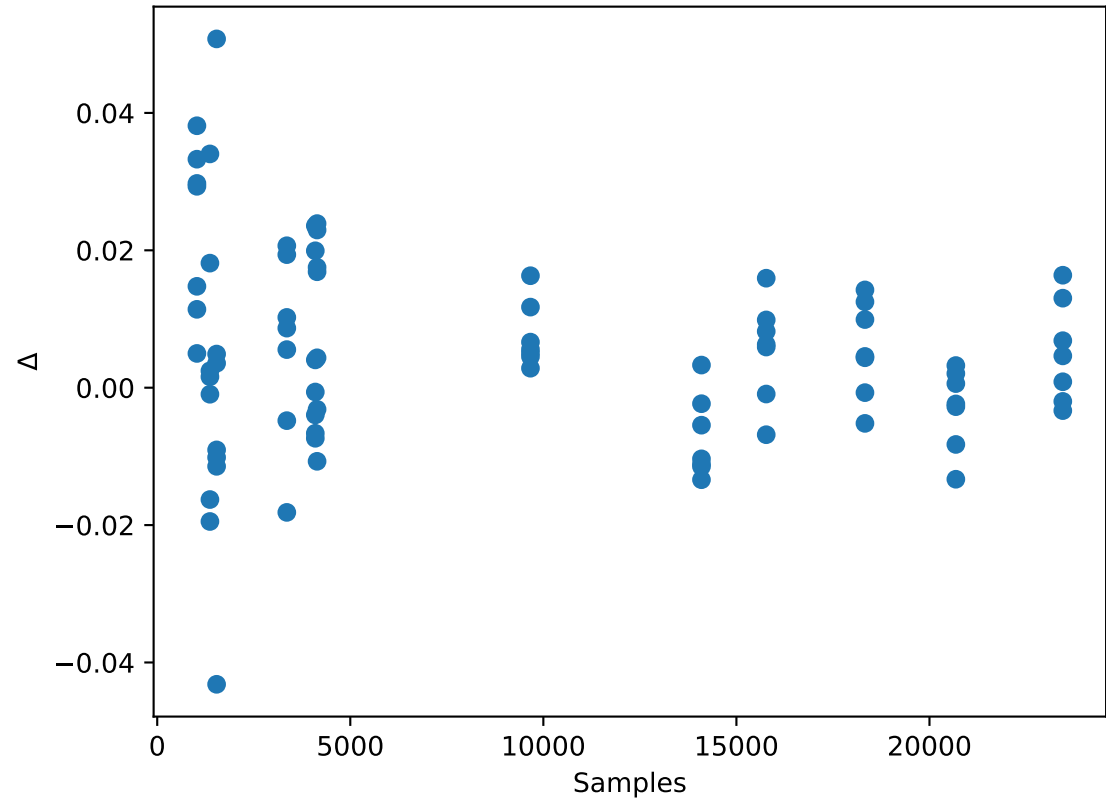
sector Samples vs \Delta - Logistic
