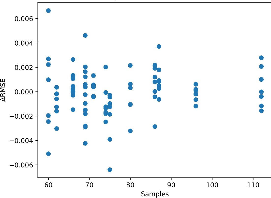
Samples vs \Delta RMSE - XGBoost
