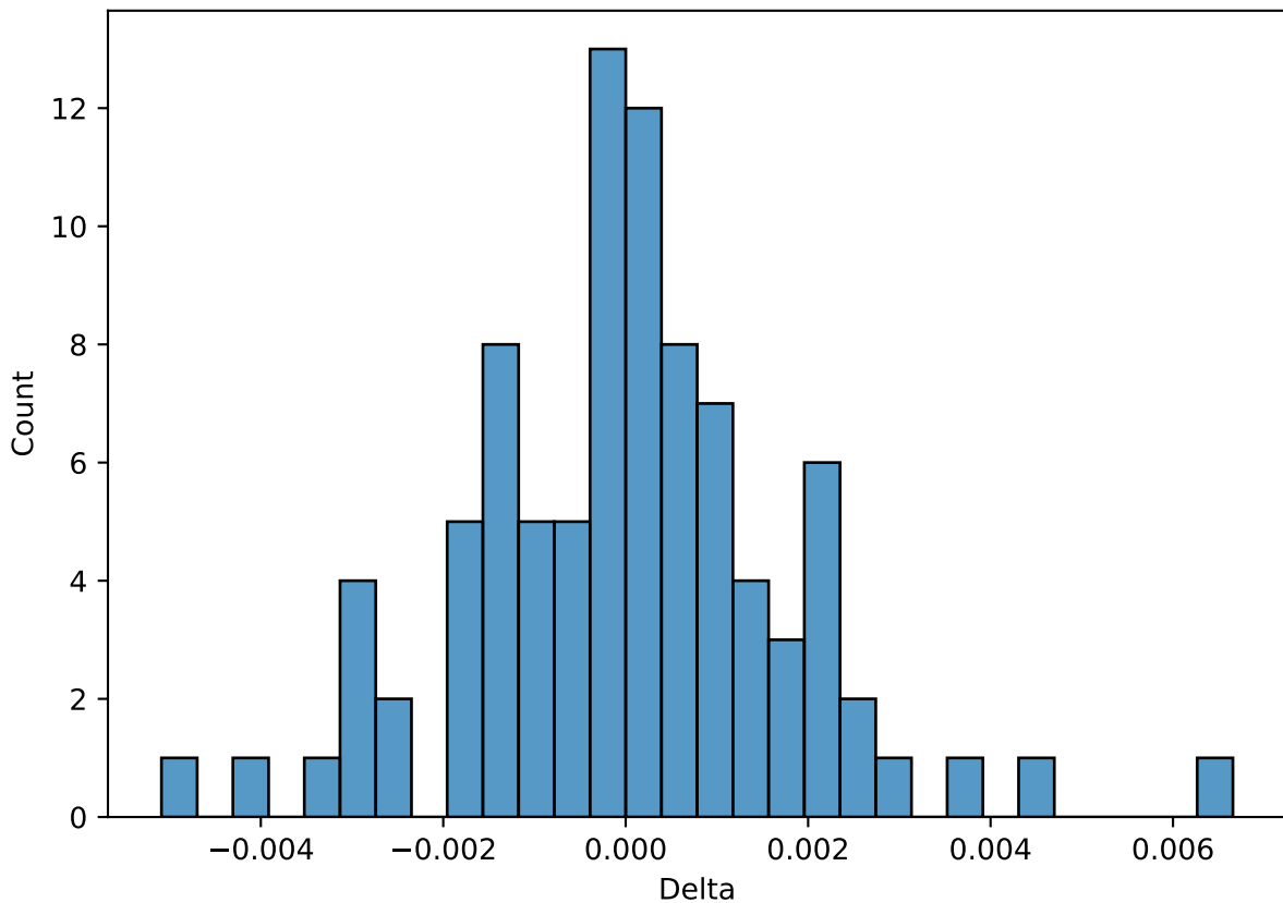
ticker \Delta Distribution - XGBoost
