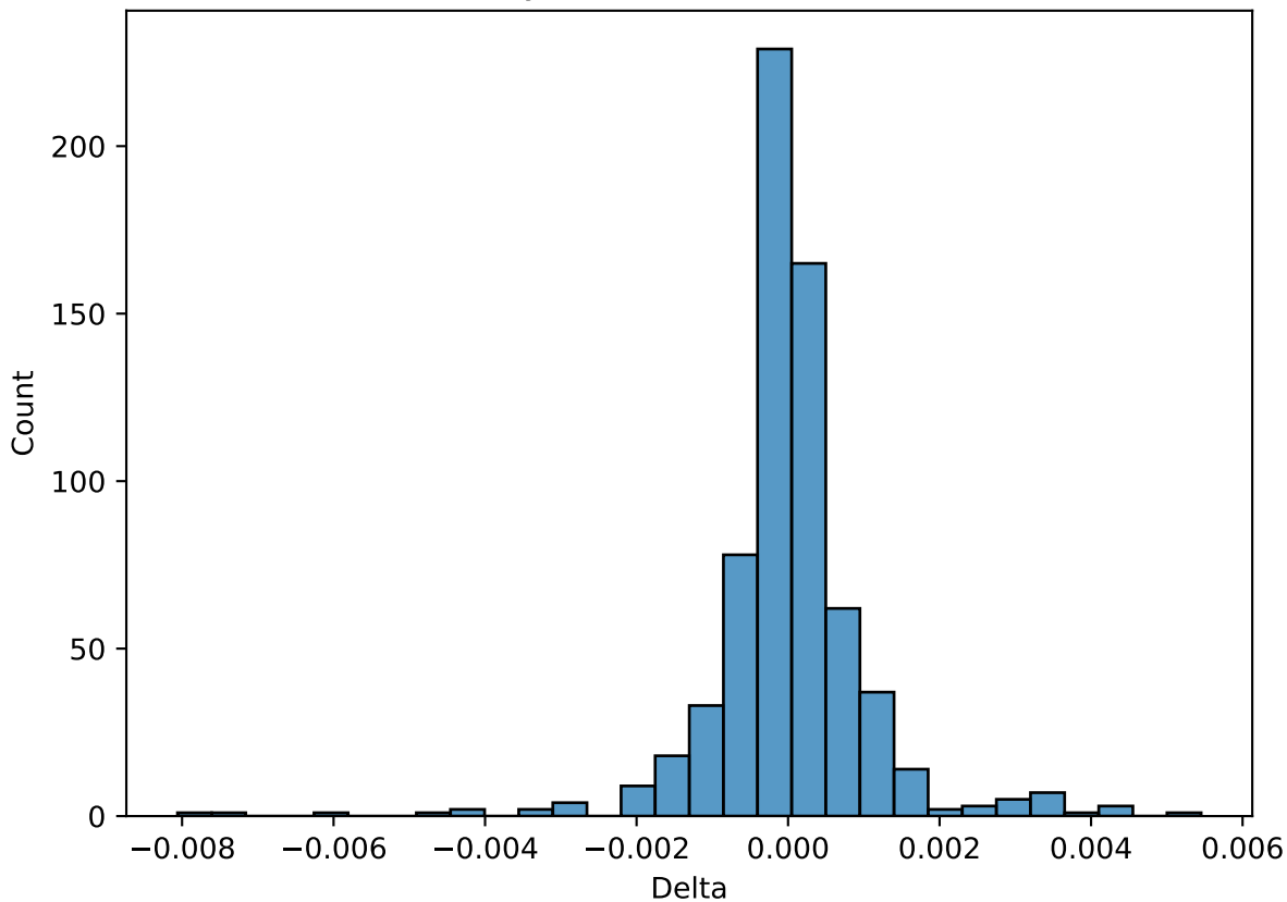
industry \Delta Distribution - XGBoost
