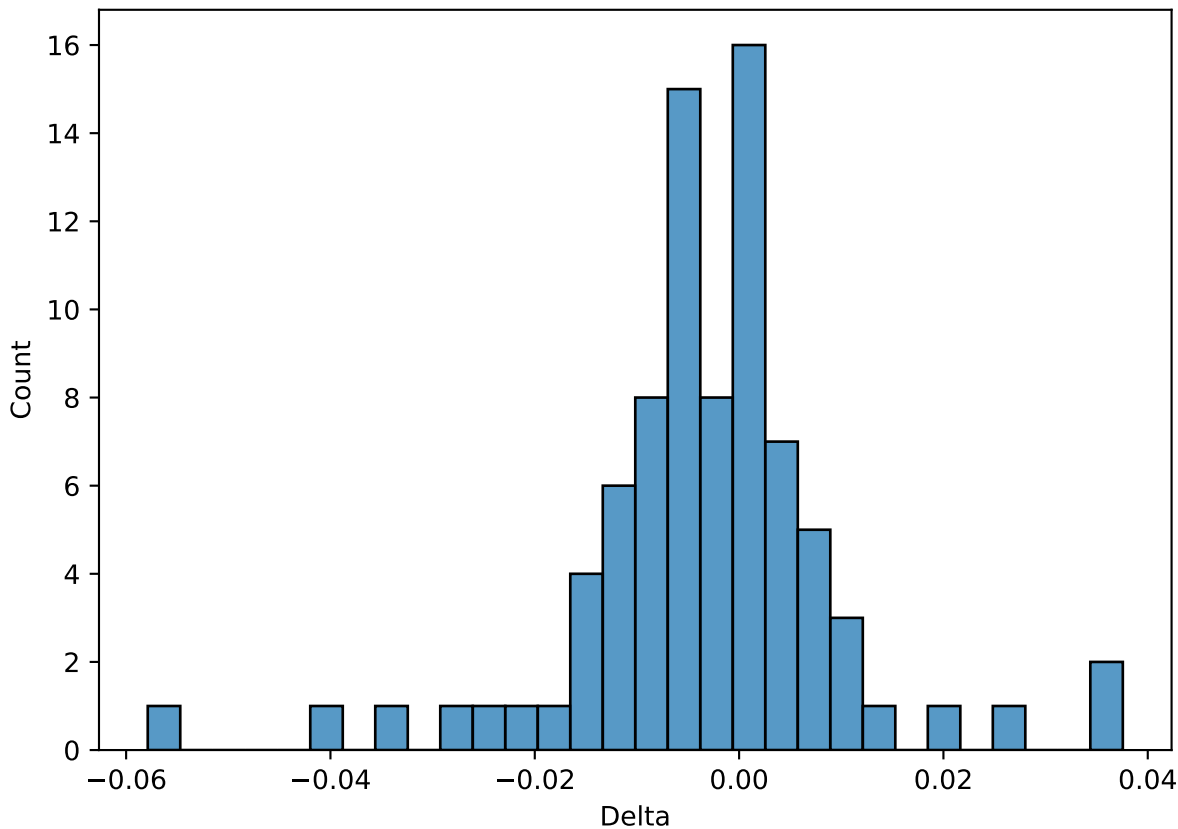
sector \Delta Distribution - XGBoost
