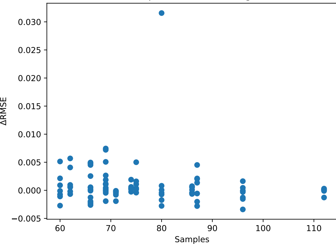
Samples vs \Delta RMSE - Ridge
