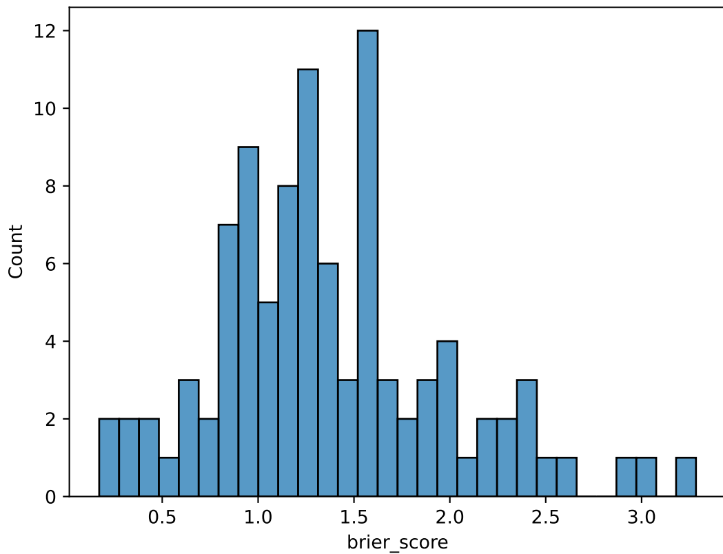
Distribution of Brier Scores
