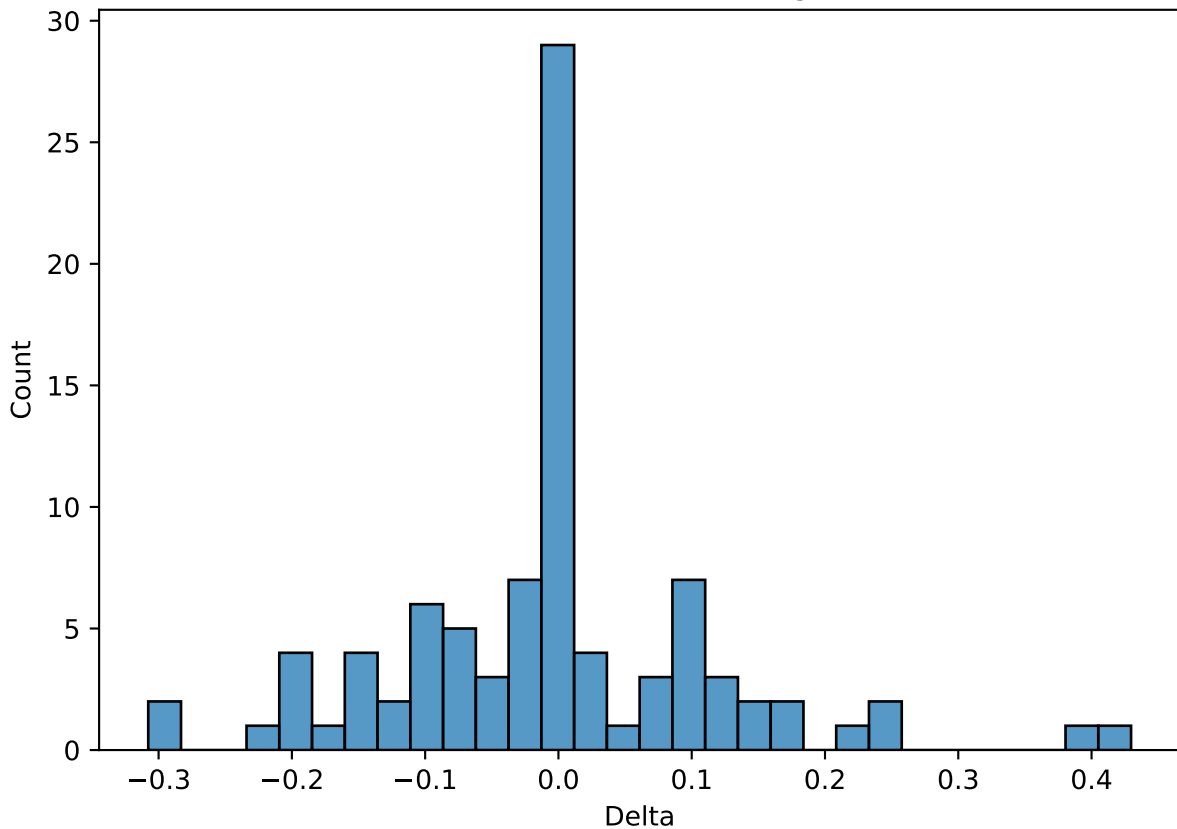
ticker \Delta Distribution - Logistic
