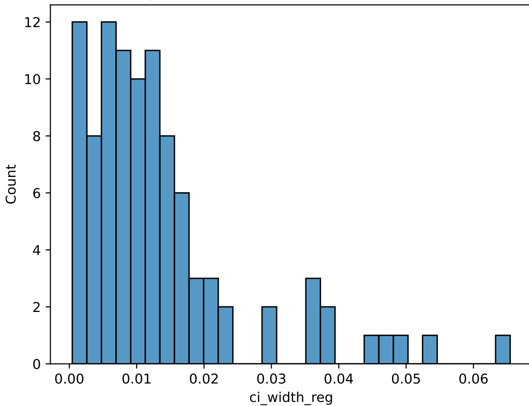
Regression CV Confidence Interval Width
