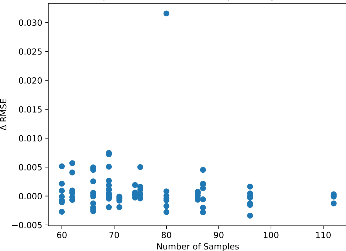
Sample Size vs Sentiment Impact (Regression)
