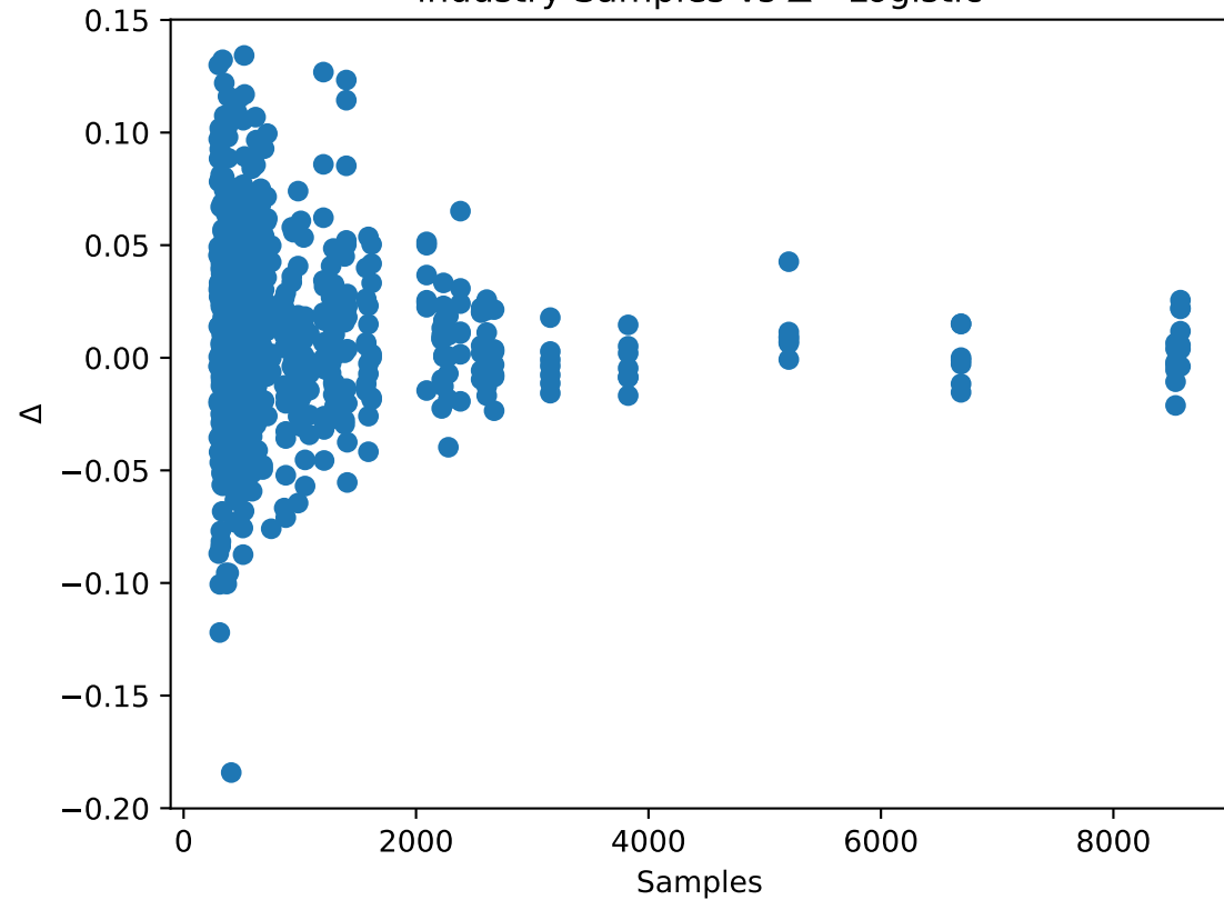
industry Samples vs \Delta - Logistic
