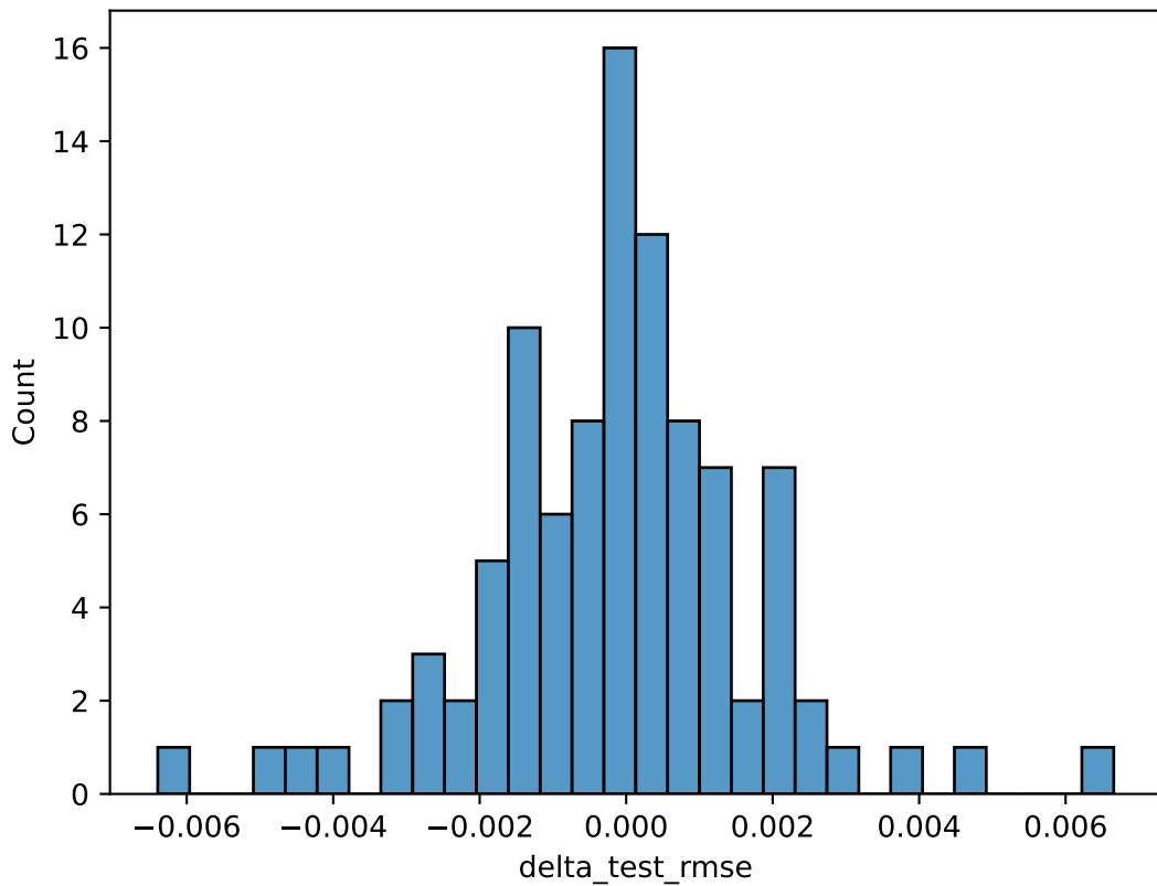
\Delta RMSE Distribution - XGBoost
