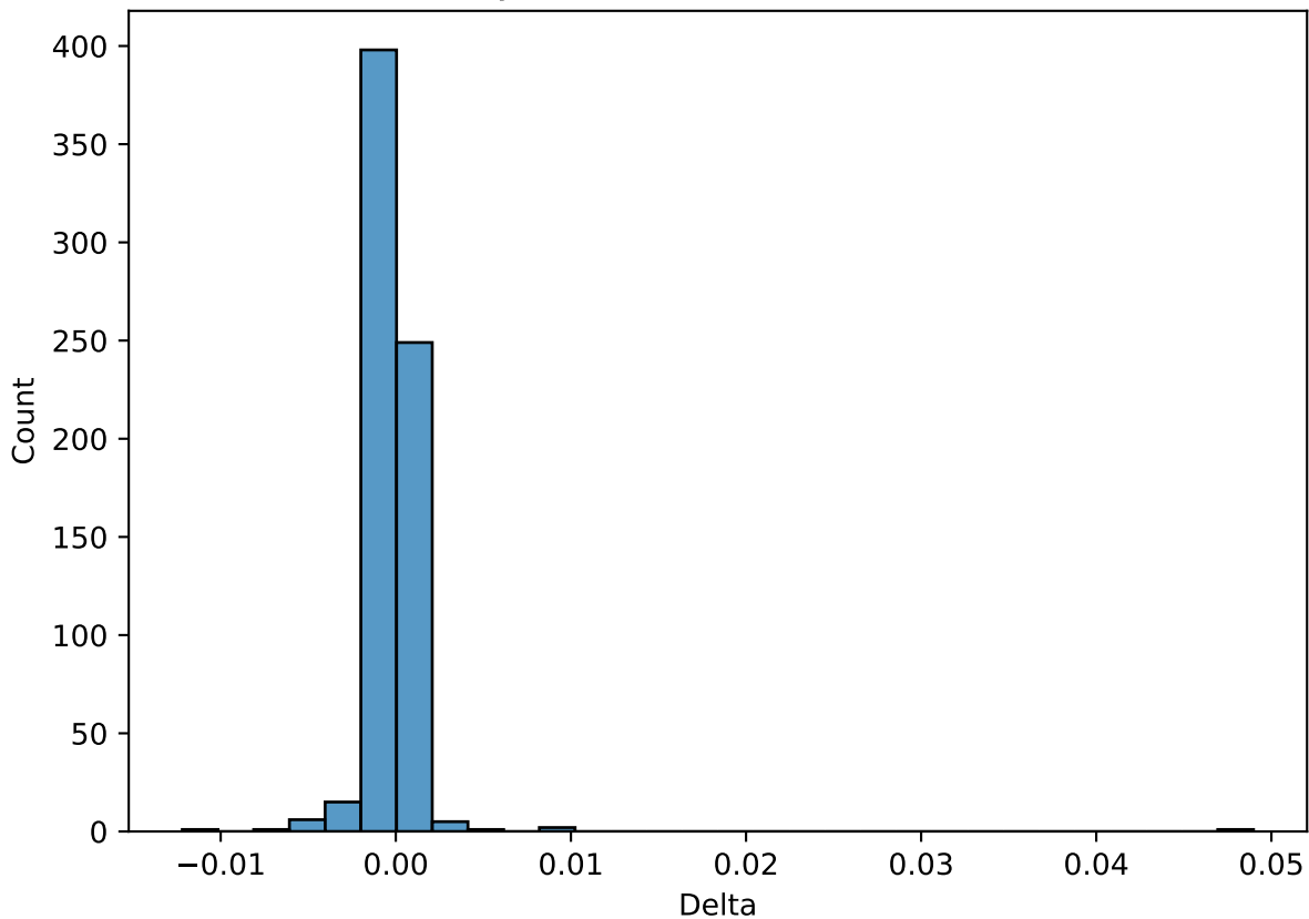
industry \Delta Distribution - RandomForest
