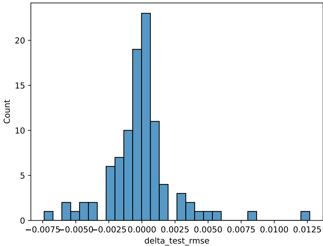
\Delta RMSE Distribution - RandomForest
