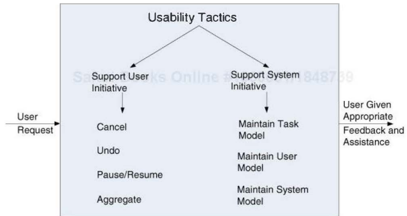
Figure 11.3. Usability tactics
