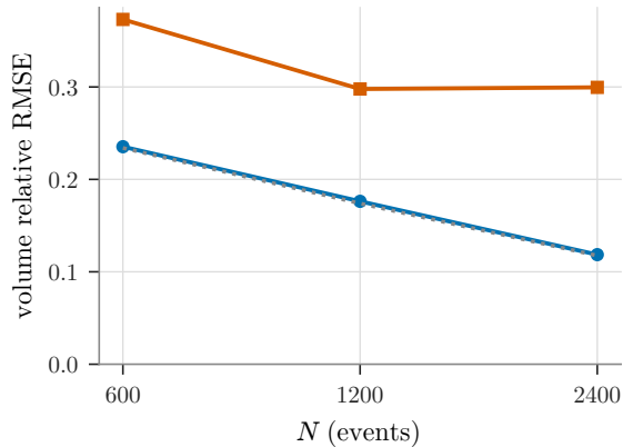
(a) floor vs recovered scaling
