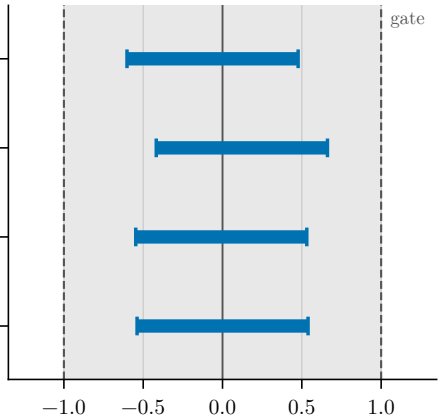
(b) equivalence gate ( \tau = 2.5\% )
