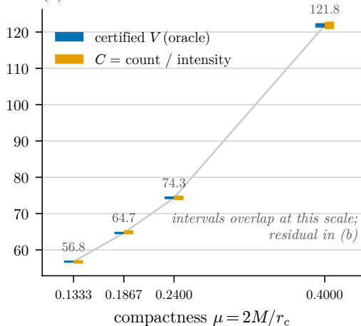
(a) certified volume vs count
