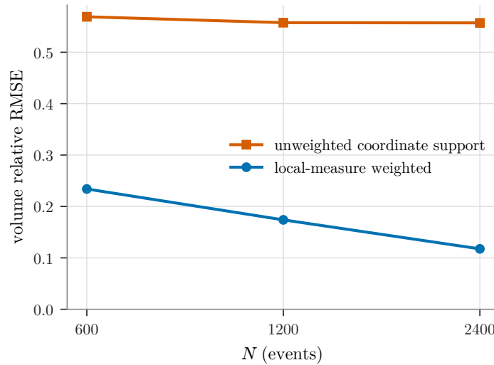
Figure 4. R5: volume reconstruction requires supplied measure information. For the coordinate-volume support sampling used in exp19 , the weighted estimate has negligible observed bias and decreasing RMSE over the tested N , while omitting the supplied local weights gives the reported persistent bias (constant-1.5 conformal profile). Equivalent measure information can conceptually be encoded in the sampling law rather than as post-hoc weights; that alternative is not part of this figure’s evidence package. Order alone fixes no absolute scale.
